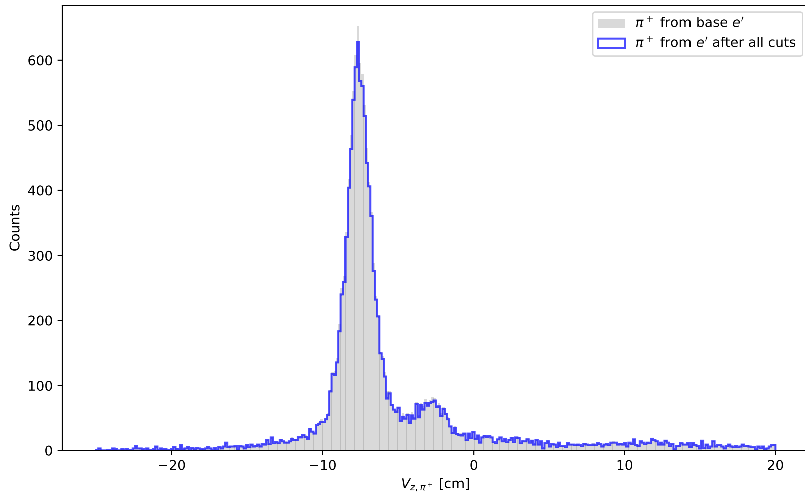
Cu Pion Vertex Distribution: V_{z,\pi^+}
