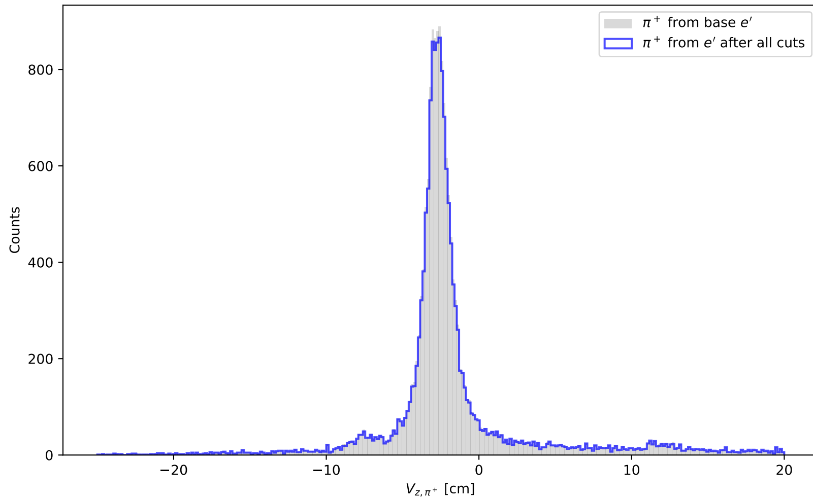
Sn Pion Vertex Distribution: V_{z,\pi^+}
