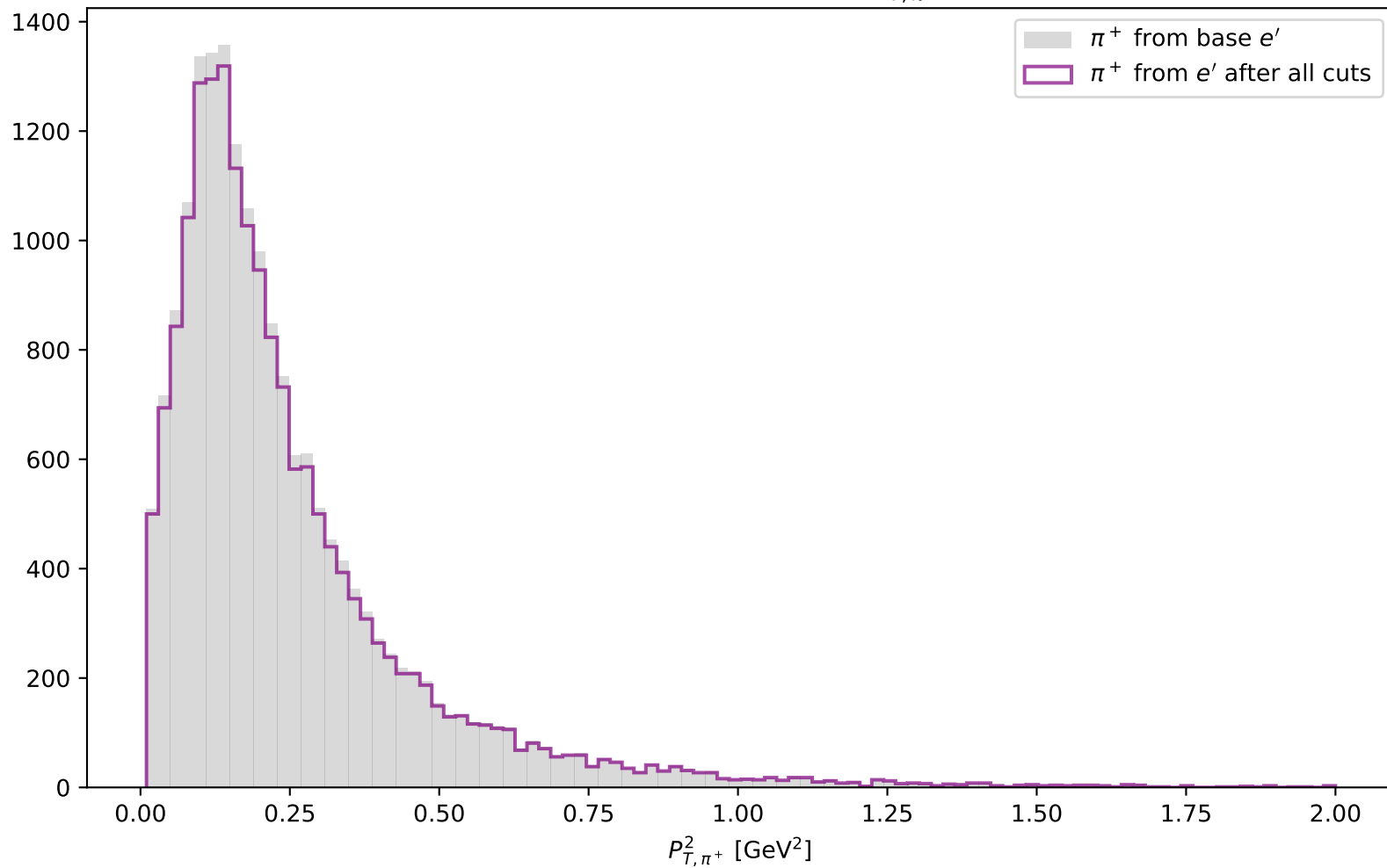
Transverse Momentum P_{T,\pi^+}^2
