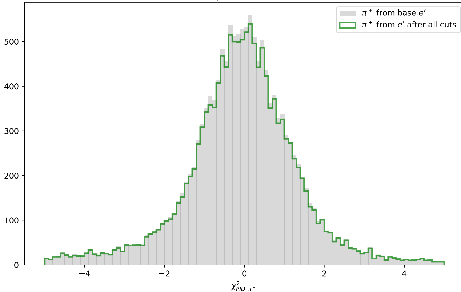
\chi^2_{PID, \pi^+} Distribution
