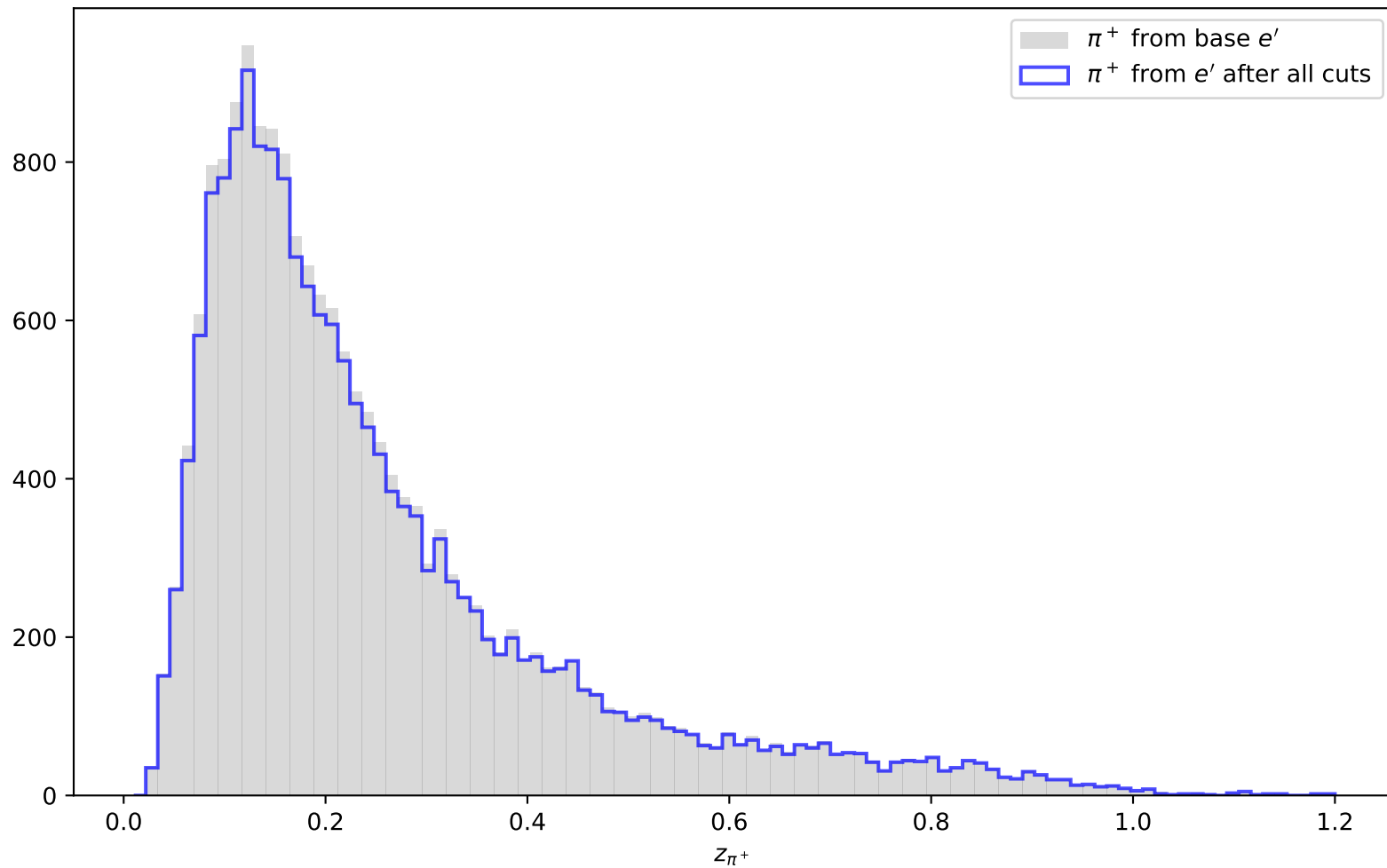
Energy Fraction z_{\pi^+}
