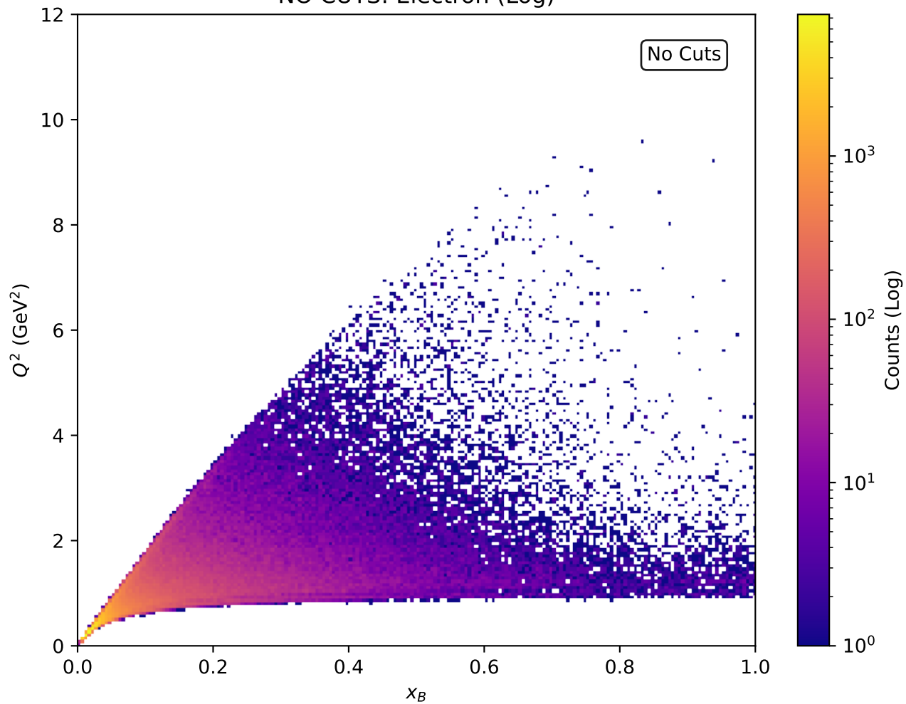
NO CUTS: Electron (Log)
