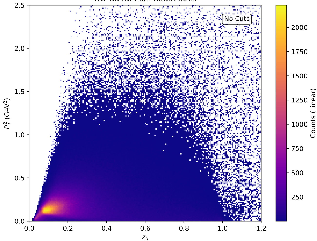
NO CUTS: Pion Kinematics
