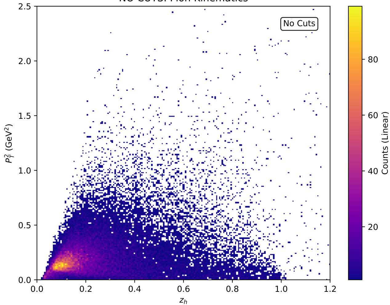
NO CUTS: Pion Kinematics
