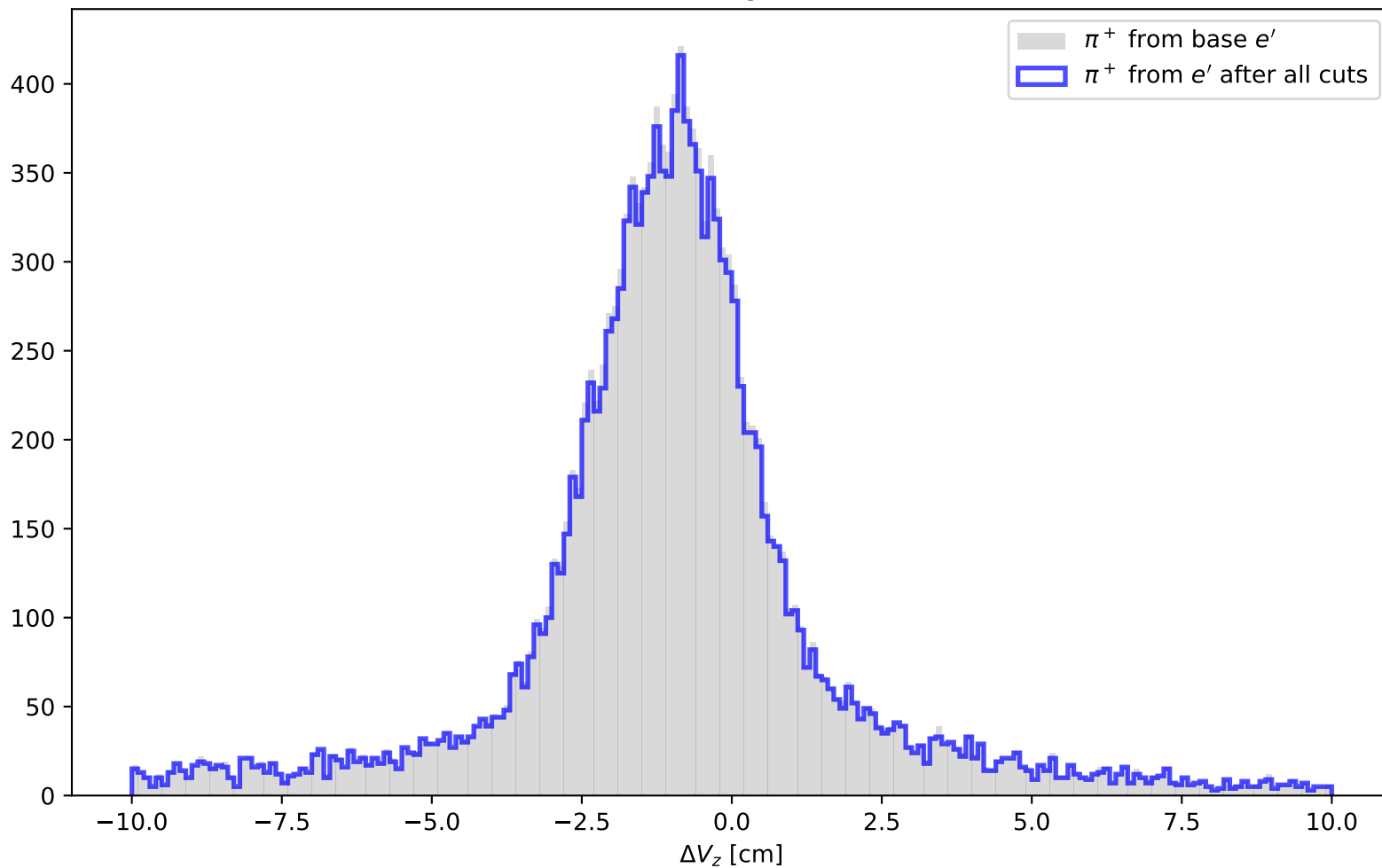
Vertex Matching: \Delta V_z(e', \pi^+)
