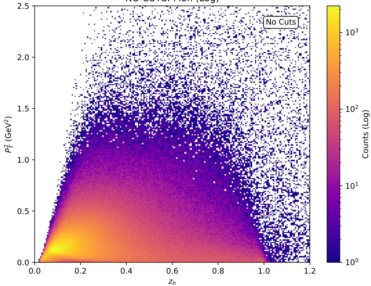
NO CUTS: Pion (Log)
