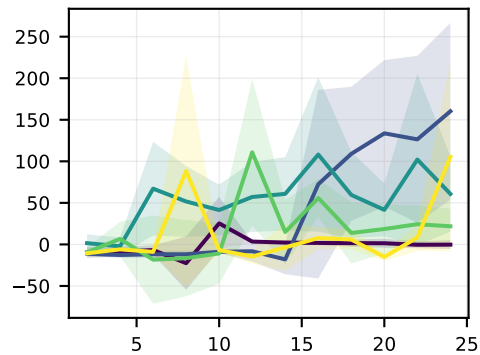
Walker2dVelocity
