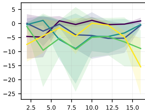
CarButton1 (new)
