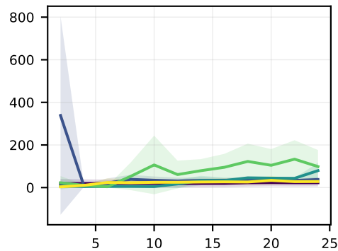
HopperVelocity
