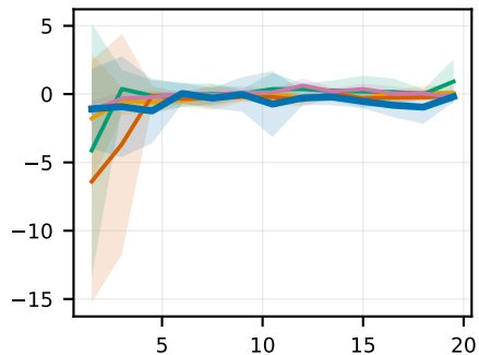
PointGoal2 (new)
