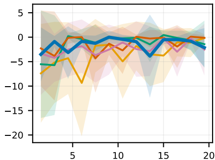
CarButton1 (new)
