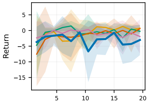
CarGoal1 (new)
