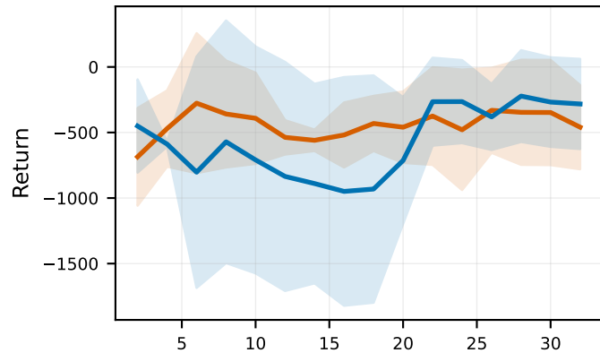
HalfCheetah / SAC-Lag (clear win: more reward, cost stays ~0)
