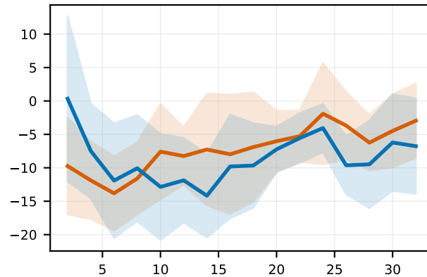
Swimmer / SAC-Lag (regression: cost up across all optimizers)
