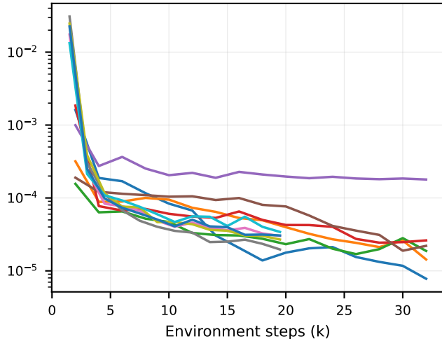
Minimax estimator loss
