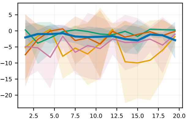
CarGoal1*
