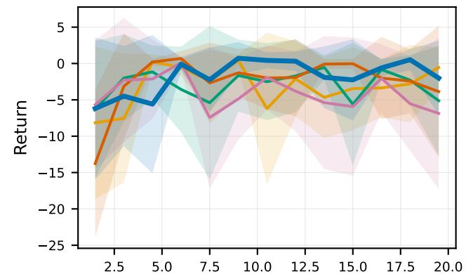
CarButton1*
