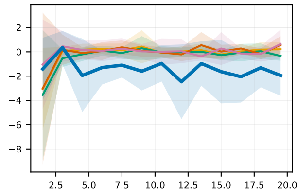
PointButton1
