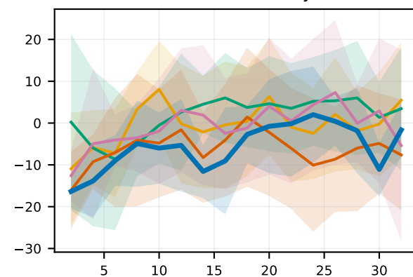
SwimmerVelocity
