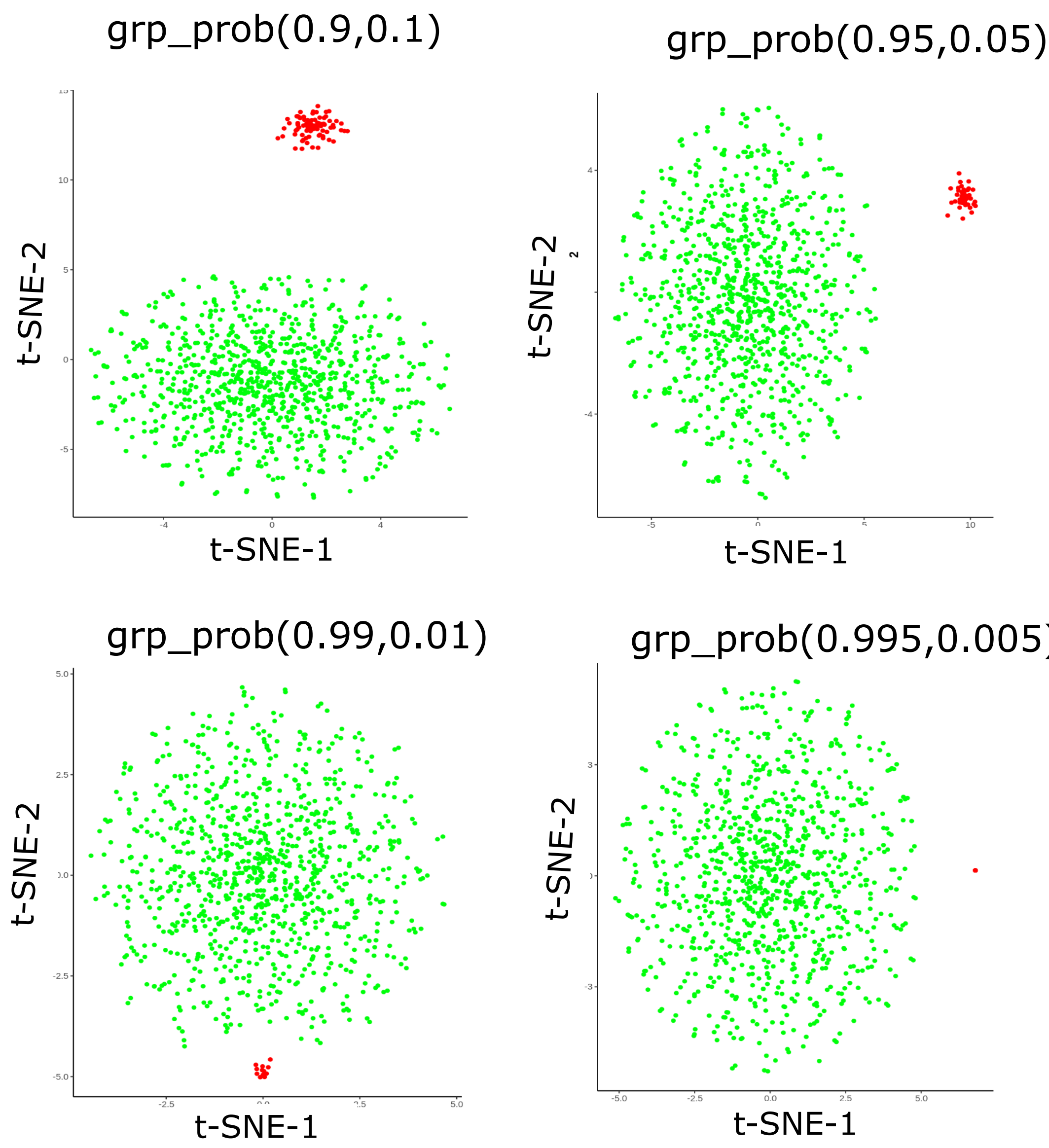
Simulation setting S1 (DE=40%, dropout rate=0.2)
