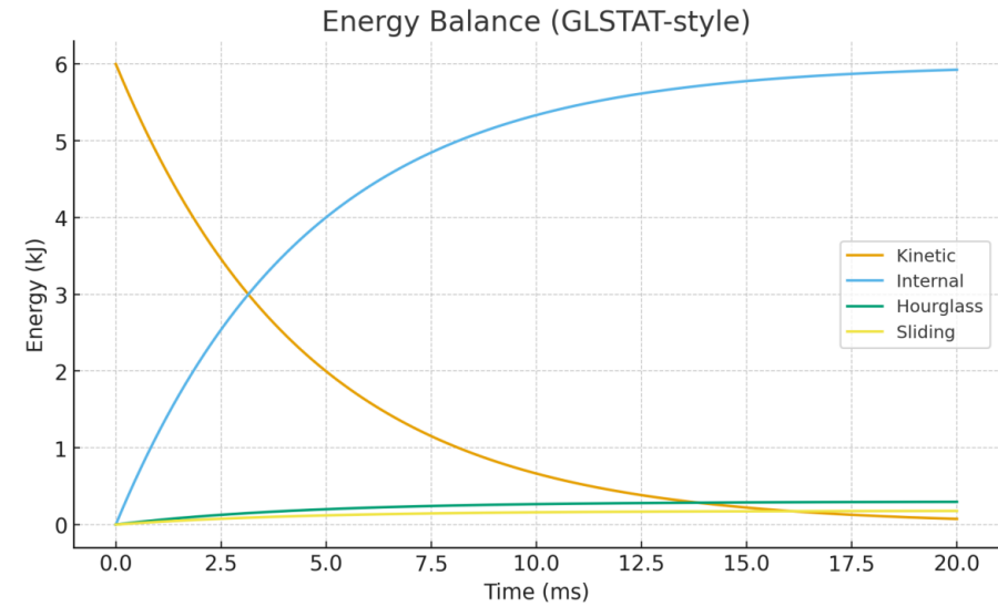
Energy Balance
