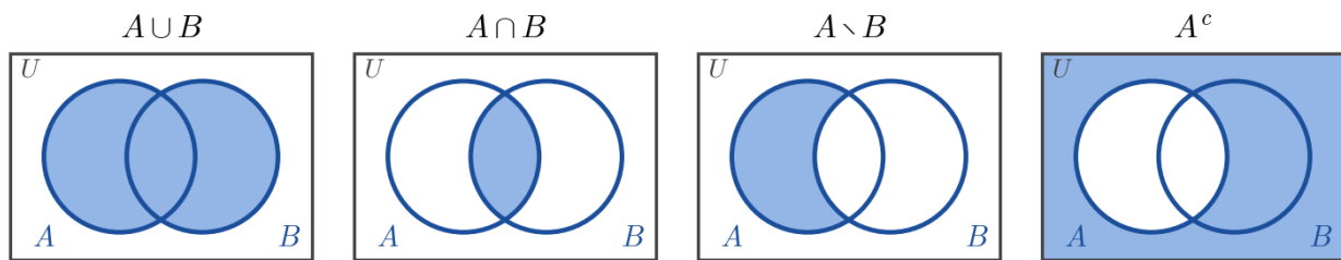
Figure 1.1.1: The four basic operations, shaded. The rectangle is the universal set U .
