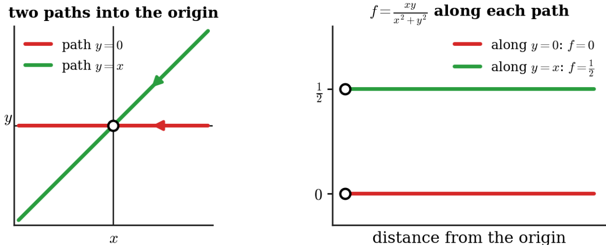
Figure 3.1.3: Approaching the origin along y = 0 and along y = x . On the left, the two paths in the domain; on the right, the value of f at each point of the path. Along either path f is constant , at 0 and at \frac{1}{2} respectively, so the two approaches disagree however close to the origin one gets.
