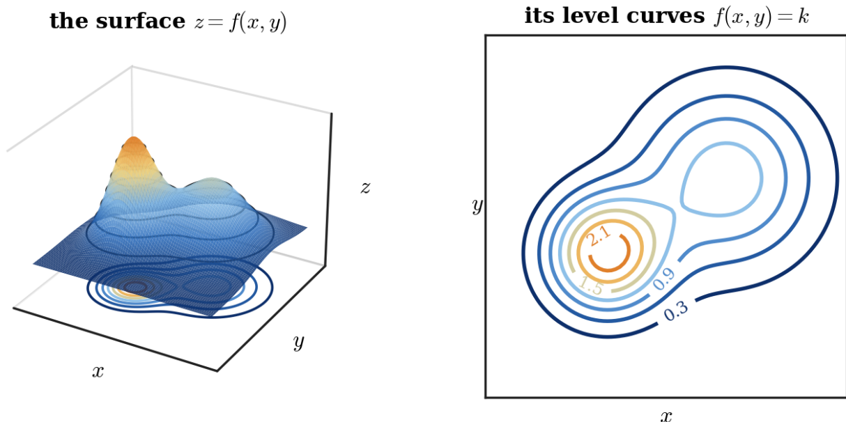
Figure 3.1.2: A surface with two peaks and its level curves. Each curve is one horizontal slice; the tightly packed curves around the taller peak show where the surface is steep.
