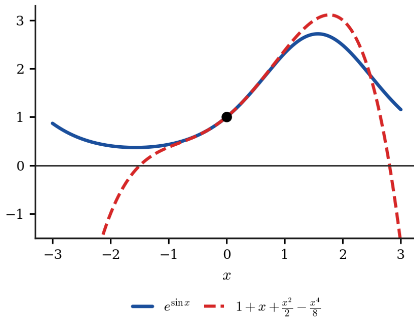
Figure 2.8.3: The fourth degree Maclaurin polynomial of e^{\sin x} is accurate near the origin and diverges from the function beyond roughly |x| > 1.5 .
