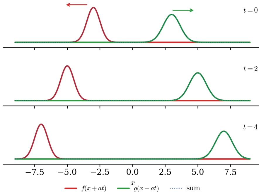
Figure 3.4.2: A solution y = f(x + at) + g(x - at) at three times. Neither bump changes shape; they simply move in opposite directions at speed a .
