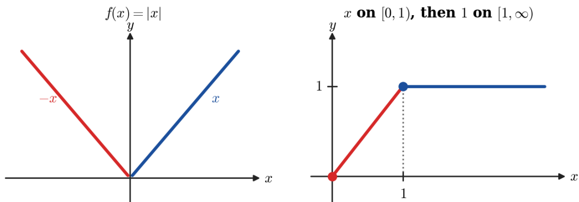
Figure 1.4.4: Two of the examples. The pieces must agree at the joins if the graph is to be unbroken there; both of these do.
