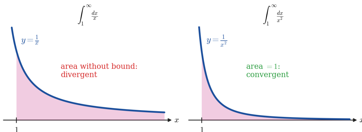
Figure 2.5.2: The two regions of the previous problems. Both are unbounded to the right and both narrow towards the axis, but only the second has finite area.
