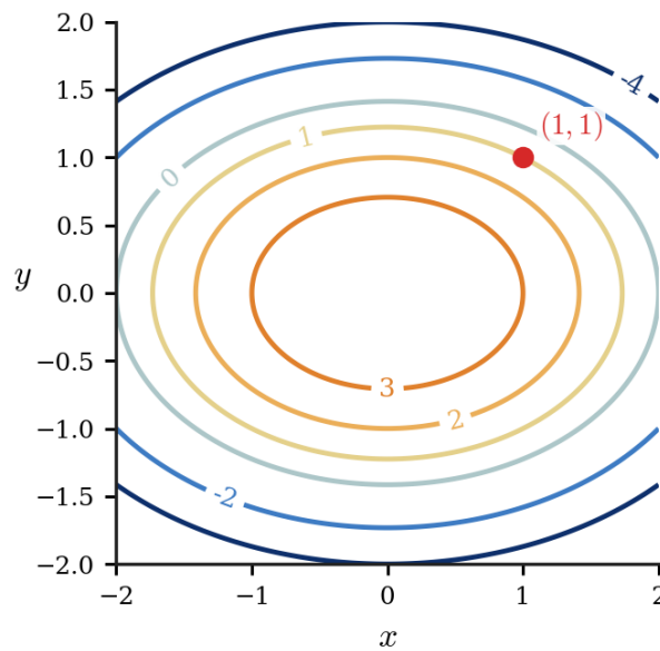
Figure 3.2.2: Level curves of f(x, y) = 4 - x^2 - 2y^2 . Both partial derivatives are negative at (1, 1) , matching the fact that the level values fall as one moves away from the origin.
