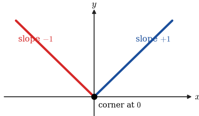
Figure 1.12.2: The graph of |x| has slope -1 on the left and +1 on the right. At the corner no single tangent line fits, so f'(0) does not exist.
