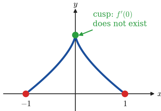
Figure 2.1.3: f(x) = 1 - x^{2/3} on [-1, 1] . The endpoint ordinates agree and the curve is unbroken, but the peak is a cusp, not a smooth maximum, so no horizontal tangent exists.
