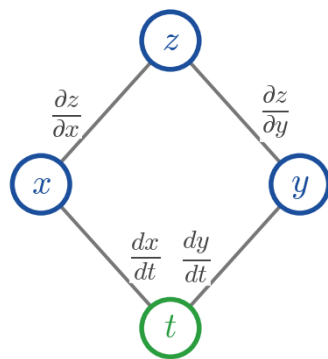
Figure 3.7.1: Reading the chain rule off a tree. Each path from the top to the bottom contributes one product, and the products are added.
