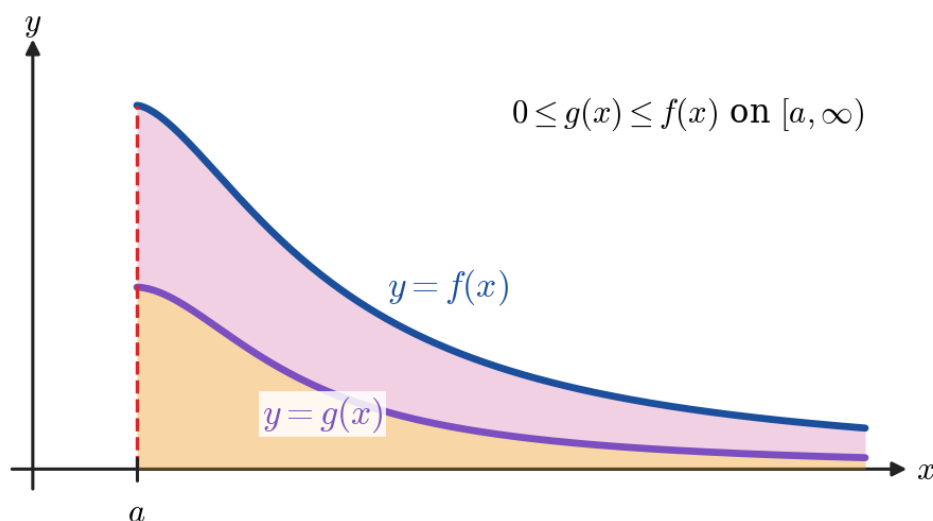
Figure 2.5.4: The graph of g lies between the x -axis and the graph of f throughout [a, \infty) , so the area under g is contained in the area under f . A finite outer area forces a finite inner one; an infinite inner area forces an infinite outer one.
