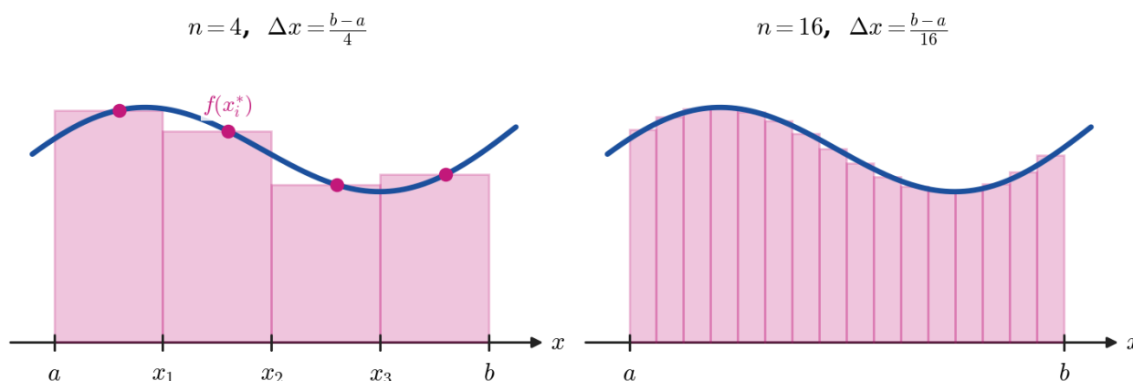
Figure 2.4.1: Riemann sums for the same function with n = 4 and n = 16 rectangles. As n increases the rectangles narrow, the staircase settles onto the curve, and the sums approach \int_a^b f(x) dx .
