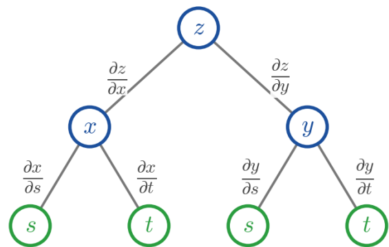
Figure 3.7.1: Reading the chain rule off a tree. Each path from the top to the bottom contributes one product, and the products are added.
