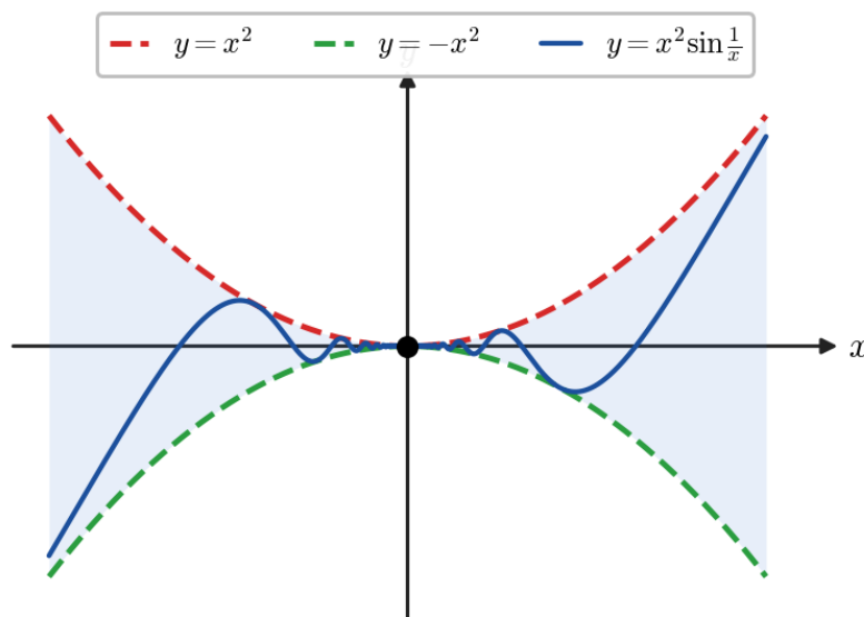
Figure 1.10.2: The oscillation is trapped between -x^2 and x^2 , which pinch together at the origin and force the limit to be 0.
