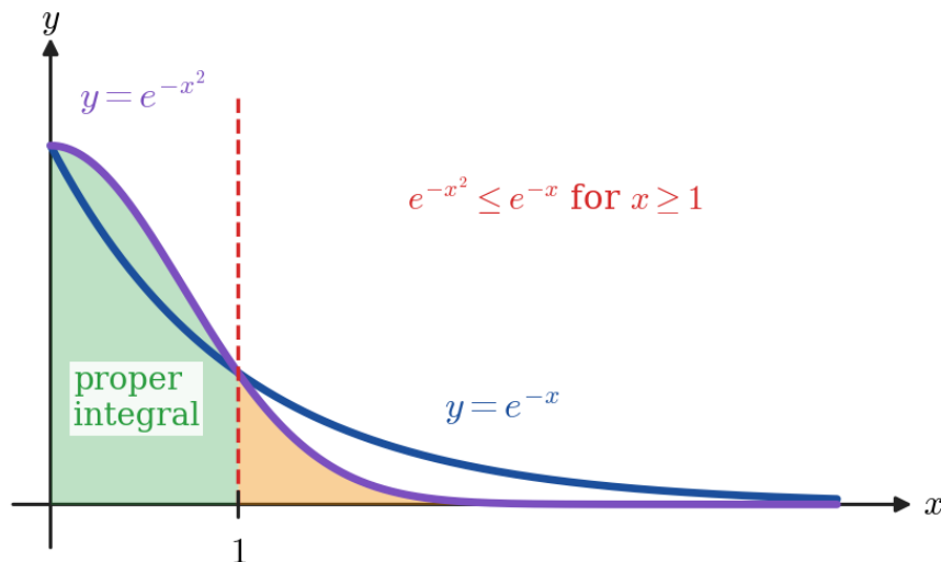
Figure 2.5.5: On [1, \infty) the curve e^{-x^2} lies below e^{-x} , so its tail area is finite. On [0, 1] the inequality runs the other way, which is exactly why that part is split off and handled as a proper integral instead.
