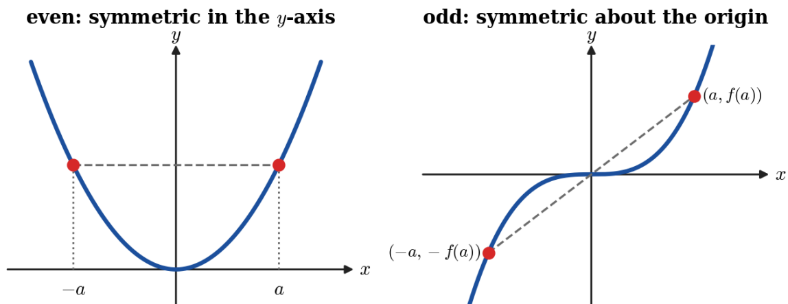
Figure 1.4.5: Even symmetry reflects the graph in the y -axis; odd symmetry turns it through half a revolution about the origin.
