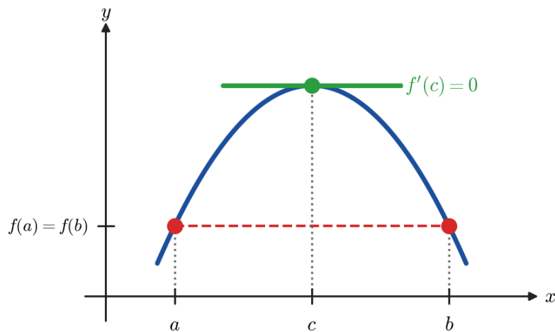
Figure 2.1.1: If the curve has equal ordinates at the ends of [a, b] , the tangent is horizontal at some interior point c .
