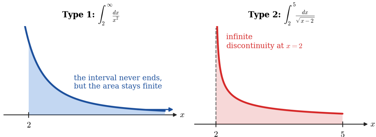
Figure 2.5.1: Two ways an integral can be improper: the region runs off to the right without ending (Type 1), or it runs upwards without ending (Type 2).
