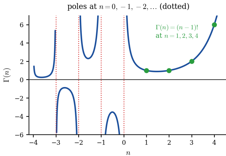
Figure 2.6.1: The gamma function. It passes through the factorials at the positive integers and has a vertical asymptote at every non-positive integer, which is where (2.6.3) breaks down.
