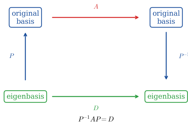
Figure 4.10.2: Diagonalisation as a change of basis. In the eigenbasis the map is the diagonal matrix D ; P and P^{-1} translate between the two bases.
