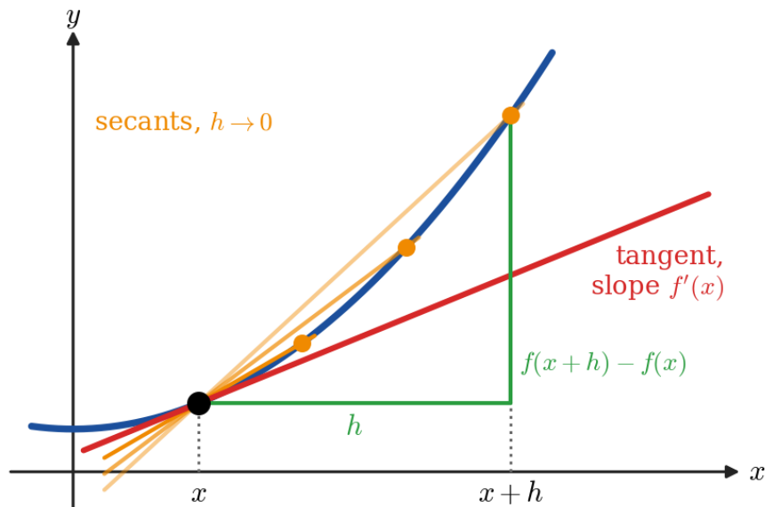
Figure 1.12.1: The quotient \frac{f(x+h) - f(x)}{h} is the slope of the secant through (x, f(x)) and (x+h, f(x+h)) . As h \rightarrow 0 the second point slides towards the first and the secants turn into the tangent, whose slope is f'(x) .
