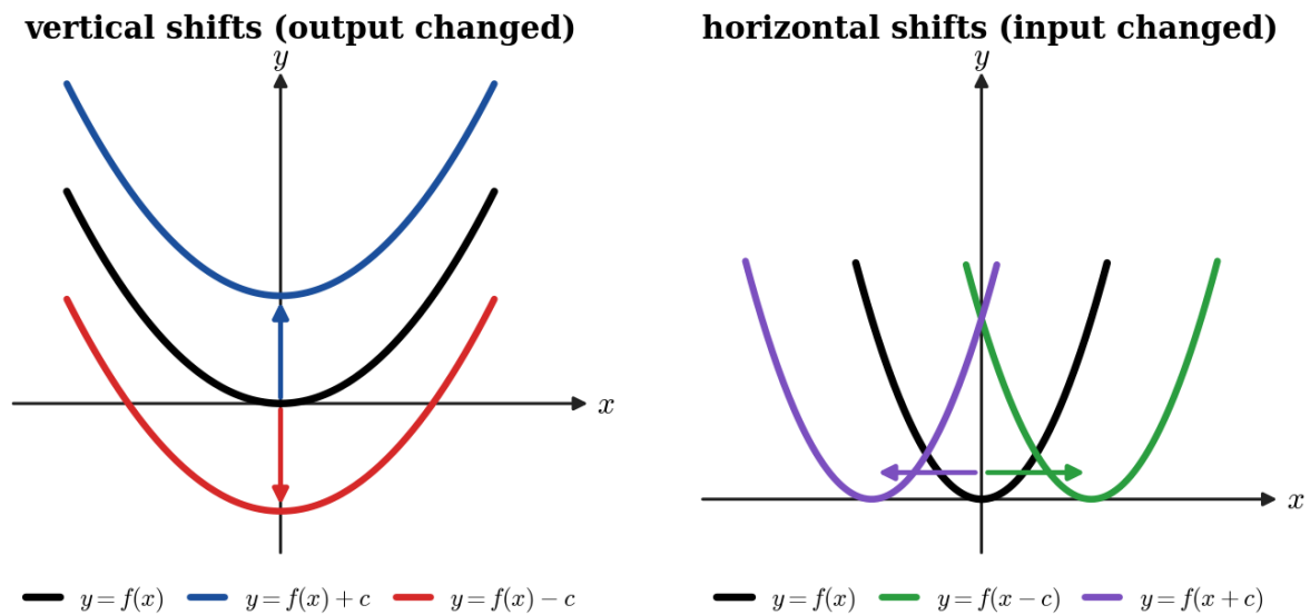
Figure 1.6.1: Left: adding c to the output moves the graph up or down. Right: replacing x by x \mp c moves it sideways — right for x - c , left for x + c .
