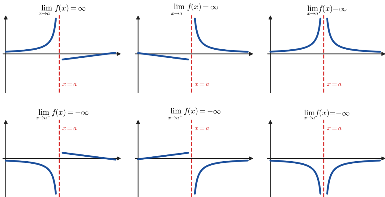
Figure 1.9.6: The six cases. Only one of them need hold for x = a to be a vertical asymptote the curve may behave quite ordinarily on the other side.
