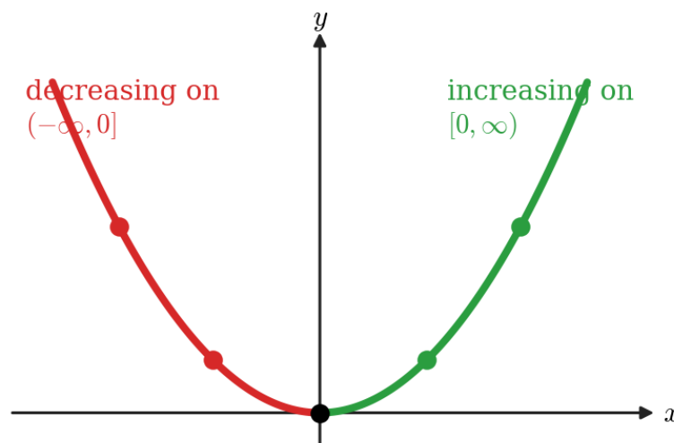
Figure 1.4.6: On the left branch, moving right lowers the height; on the right branch it raises it. A function need not be increasing or decreasing on the whole of its domain.
