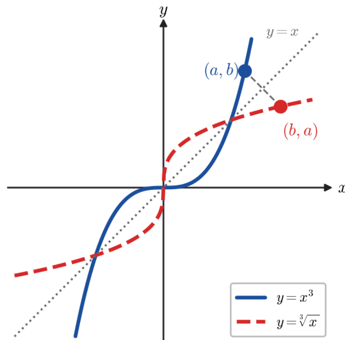
Figure 1.8.2: y = x^3 and y = \sqrt[3]{x} are mirror images in the dotted line y = x . The point (a, b) on one corresponds to (b, a) on the other.
