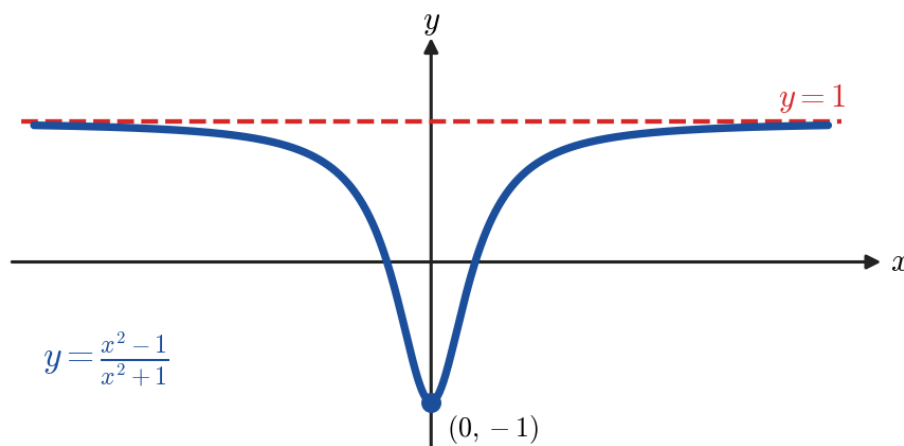
Figure 1.9.7: The curve settles towards the line y = 1 in both directions without ever reaching it.
