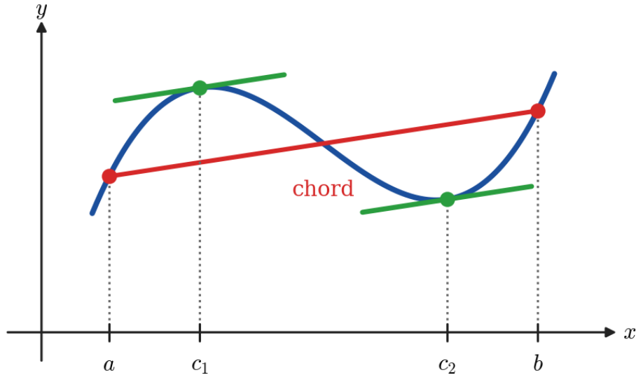
Figure 2.2.2: Two interior points at which the tangent is parallel to the chord. As with Rolle's theorem, the point c where f'(c) = \frac{f(b)-f(a)}{b-a} need not be unique.
