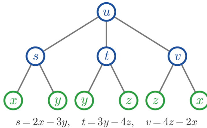
Figure 3.7.2: Each intermediate variable depends on only two of x , y , z . The branches that are absent are what removes a term from each derivative.
