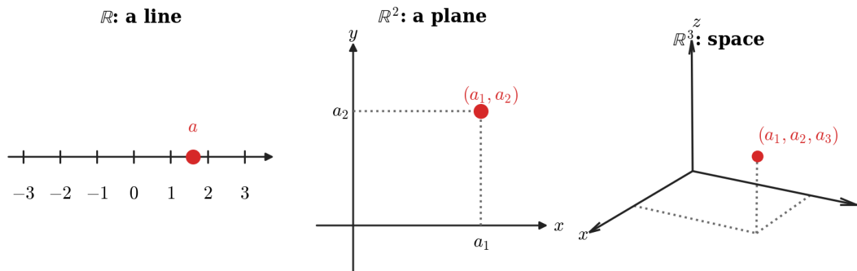
Figure 1.3.1: One coordinate gives a line, two give a plane, three give space. Each new coordinate adds a direction perpendicular to all the previous ones.
