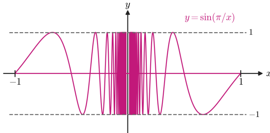
Figure 1.9.4: The oscillations crowd together without diminishing as x \rightarrow 0 , so no value of L can be approached.
