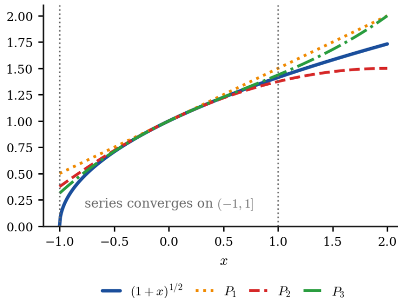
Figure 2.8.5: The binomial series for (1+x)^{1/2} . Successive partial sums approach the function on (-1, 1) and separate from it outside.
