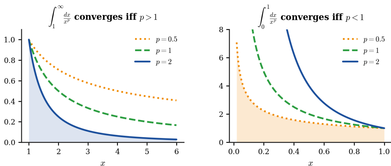
Figure 2.5.3: The same family of curves on the two intervals. The shaded region is finite in each panel: p = 2 on the left, p = \frac{1}{2} on the right.
