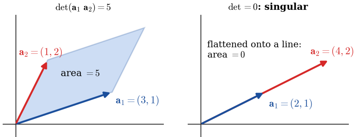
Figure 4.4.1: The absolute value of a 2 \times 2 determinant is the area of the parallelogram spanned by the columns. When the columns lie on one line the parallelogram collapses and the determinant is 0 — the matrix is singular.
