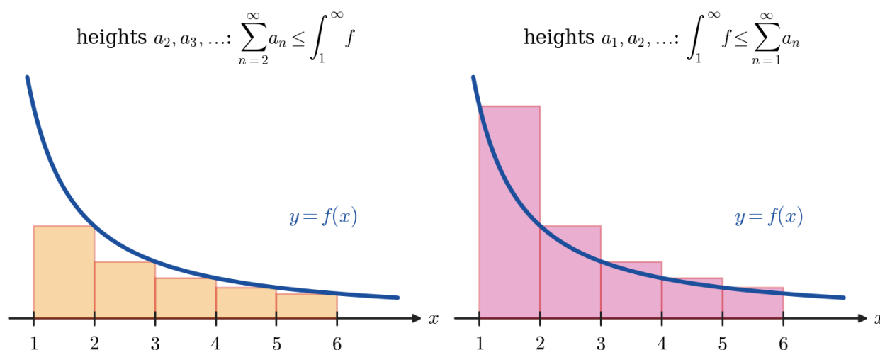
Figure 2.7.2: Rectangles of unit width and height a_n against the curve y = f(x) . Inscribed on the left, circumscribed on the right. The series and the integral trap each other between the two pictures, so neither can be finite without the other.
