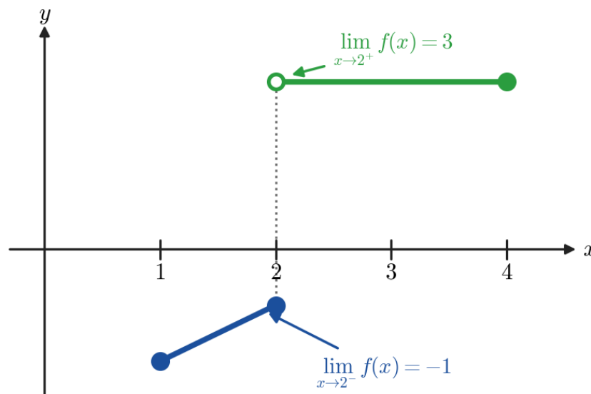
Figure 1.9.1: Approaching x = 2 from the left, the values approach -1 ; approaching from the right, they approach 3 . The filled dot marks the value f(2) = -1 that the function actually takes; the open dot marks a height that is approached but never attained.
