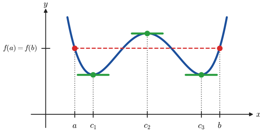
Figure 2.1.2: Rolle's theorem guarantees at least one horizontal tangent, but there may be several. Here f'(c_1) = f'(c_2) = f'(c_3) = 0 , and the theorem names none of them in particular.
