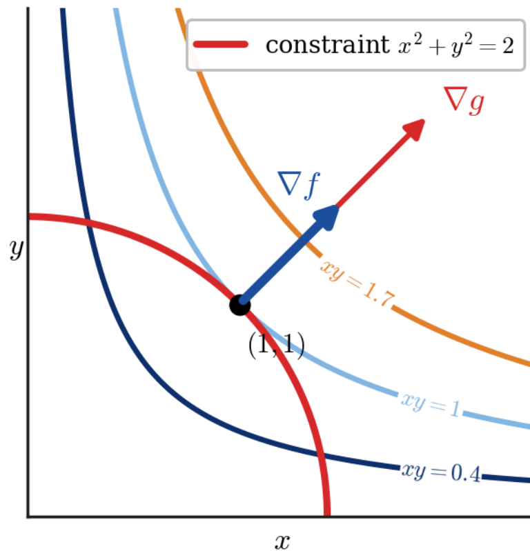
Figure 3.9.1: Why the method works, shown in two variables: maximising f = xy on the circle g = x^2 + y^2 = 2 . Moving along the circle, f increases until its level curve just touches the circle, at (1, 1) . There the two curves share a tangent, so their normals \nabla f = (1, 1) and \nabla g = (2, 2) are parallel: \nabla f = \lambda \nabla g with \lambda = \frac{1}{2} .
