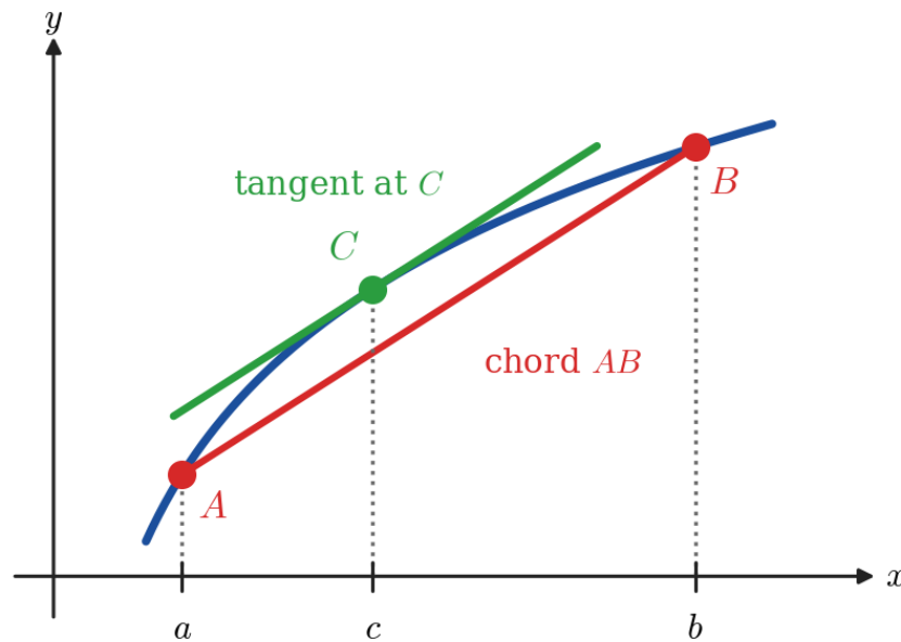
Figure 2.2.1: The tangent at c is parallel to the chord AB , whose slope is m_{AB} = \frac{f(b) - f(a)}{b - a} .
