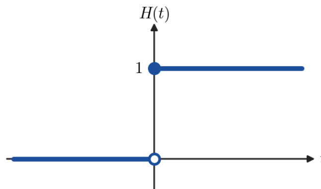
Figure 1.9.5: A jump of size 1 at the origin. The one-sided limits both exist but differ.
