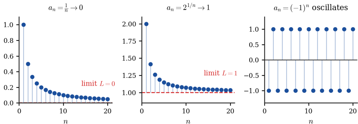
Figure 2.7.1: A sequence is defined only at integer values of n . The first two settle down to a limit; the third oscillates between -1 and 1 and so has no limit.
