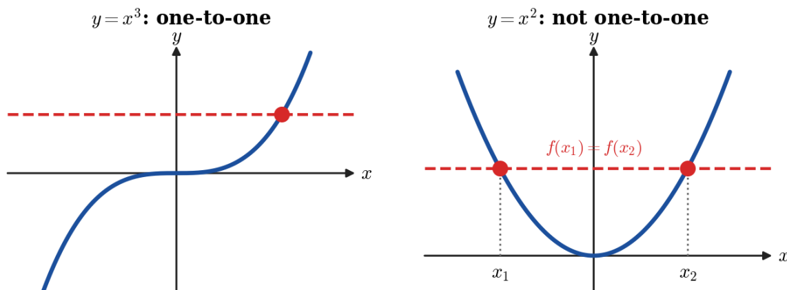
Figure 1.8.1: If a horizontal line meets the graph twice, at x_1 and x_2 , then x_1 \neq x_2 but f(x_1) = f(x_2) , and the function is not one-to-one.
