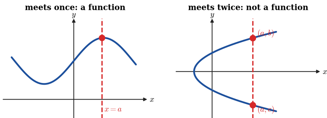
Figure 1.4.3: The vertical line x = a meets the first curve once, so each input has a single output. It meets the second twice, so a would be assigned two different values.
