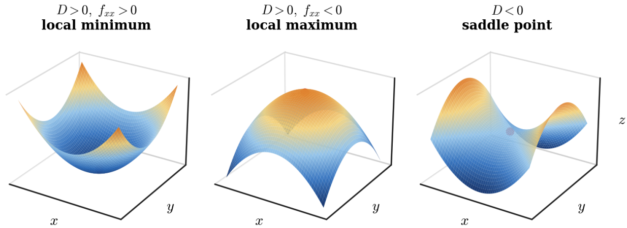
Figure 3.8.1: The three outcomes of the test at a critical point. When D > 0 the surface curves the same way in every direction, and the sign of f_{xx} says which way; when D < 0 it curves upward in one direction and downward in another.
