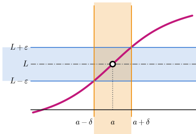
Figure 1.9.2: Given the horizontal band of half-width \varepsilon about L , a vertical band of half-width \delta about a can be found narrow enough that the graph stays inside the horizontal band.
