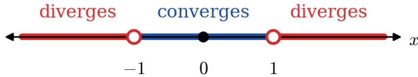
Figure 2.7.4: The series converges exactly on the open interval (-1, 1) . The endpoints are excluded: there the root test is inconclusive, but the n th term test gives divergence.
