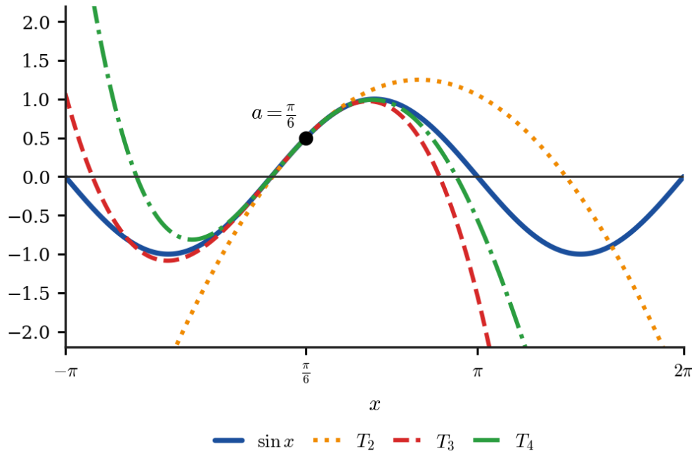
Figure 2.8.2: Successive Taylor polynomials of \sin x about a = \pi/6 . Each extra term widens the stretch over which the polynomial follows the curve, but every one of them eventually leaves it.
