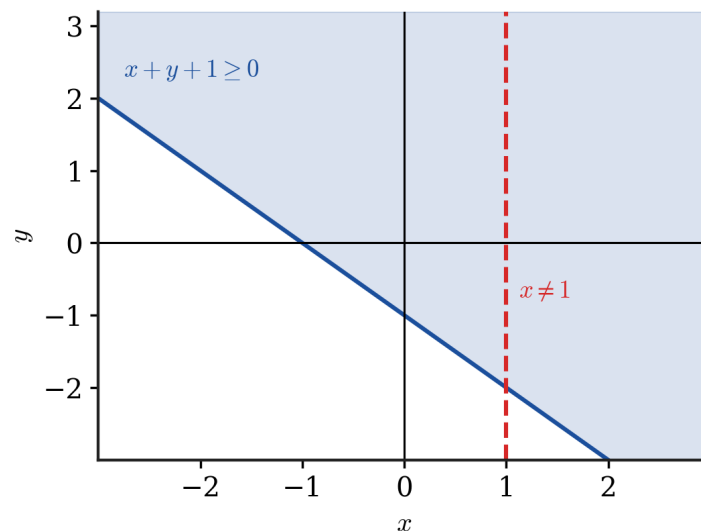
Figure 3.1.1: Domain of f(x, y) = \frac{\sqrt{x+y+1}}{x-1} . For a function of two variables the domain is a region of the plane, not an interval.
