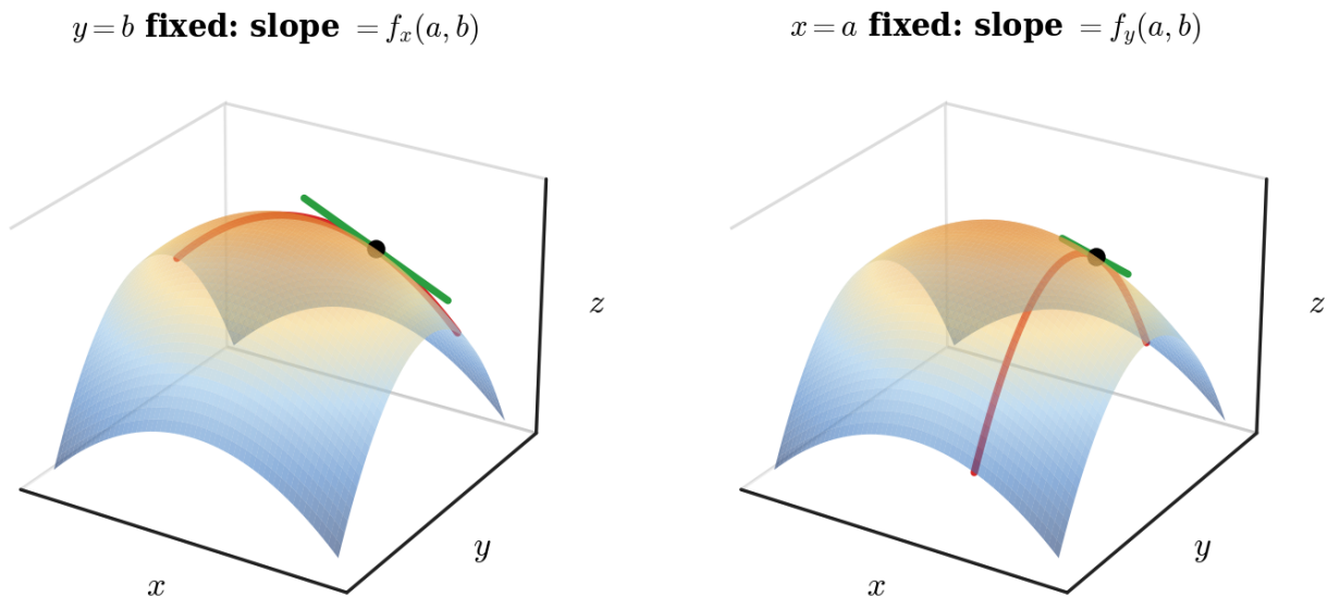
Figure 3.2.1: Each partial derivative is an ordinary derivative along one slice. The plane cuts a curve out of the surface (in red) and the partial derivative is the slope of the tangent to that curve (in green).
