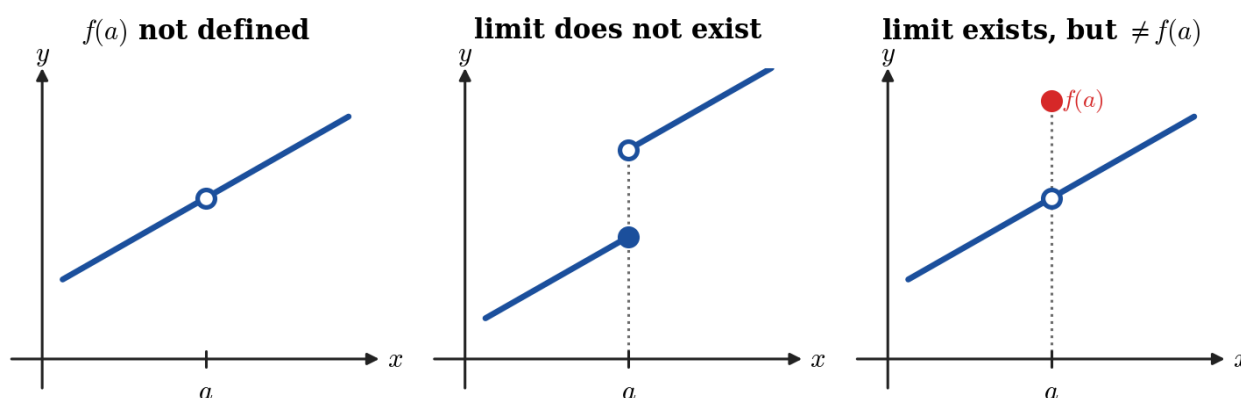
Figure 1.10.1: The three ways continuity can fail at a . Only in the middle case does the limit itself not exist.
