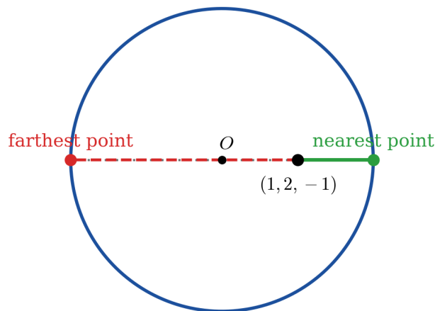
Figure 3.9.4: The plane section through the centre and the given point. Both extreme points lie on the line joining the centre to (1, 2, -1) , which is what the three Lagrange equations force.
