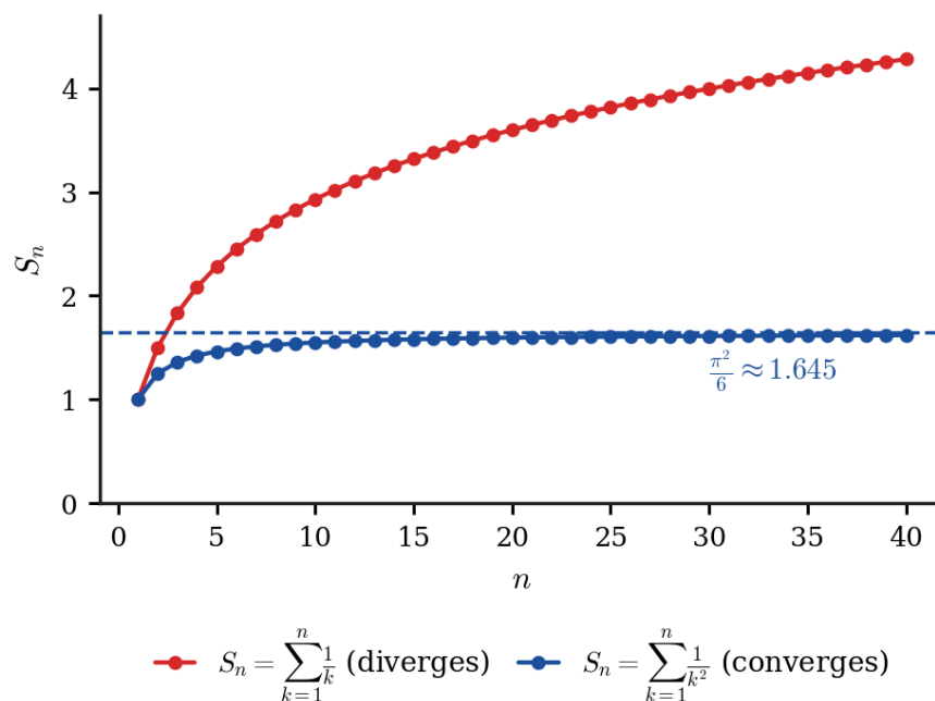
Figure 2.7.3: Partial sums of \sum \frac{1}{k} keep climbing without bound, while those of \sum \frac{1}{k^2} level off at \pi^2/6 .
