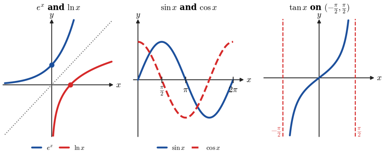
Figure 1.5.2: Left: e^x and \ln x are mirror images in the line y = x , because each undoes the other. Centre: \sin x is odd and \cos x is even. Right: \tan x has vertical asymptotes wherever \cos x = 0 .
