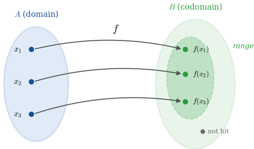
Figure 1.4.1: A function f : A \rightarrow B . Every element of A has exactly one arrow leaving it. The range is the part of B actually hit, and may be smaller than B .
