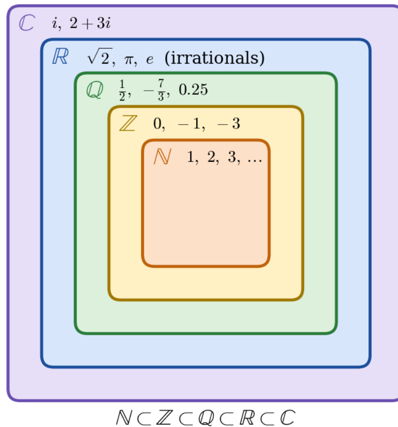
Figure 1.2.1: The number systems nested. Each ring holds numbers the ring inside it cannot express.
