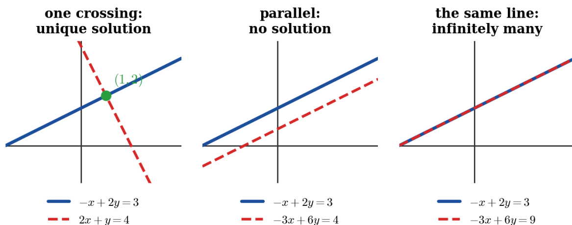
Figure 4.8.1: The three possibilities, drawn for two equations in two unknowns. Each equation is a line, and the solution set is the intersection.
