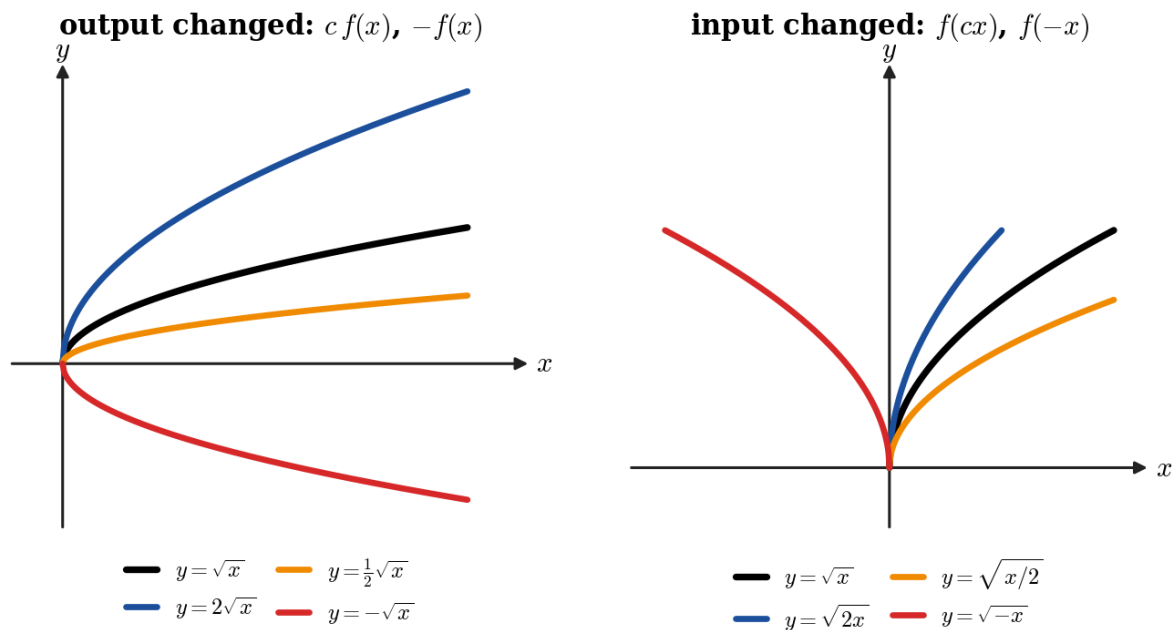
Figure 1.6.2: Shown for f(x) = \sqrt{x} with c = 2 . Left: multiplying the output scales the graph vertically, and -f(x) flips it in the x -axis. Right: f(2x) is compressed horizontally, f(x/2) is stretched, and f(-x) is flipped in the y -axis.
