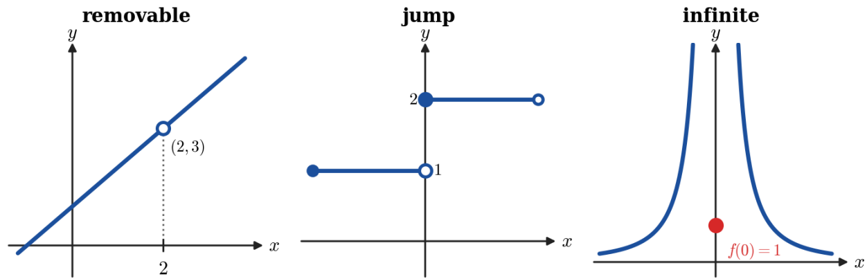
Figure 1.11.1: The three types, drawn on the functions of the worked problems below. Only the removable one can be repaired by changing the function at a single point.
