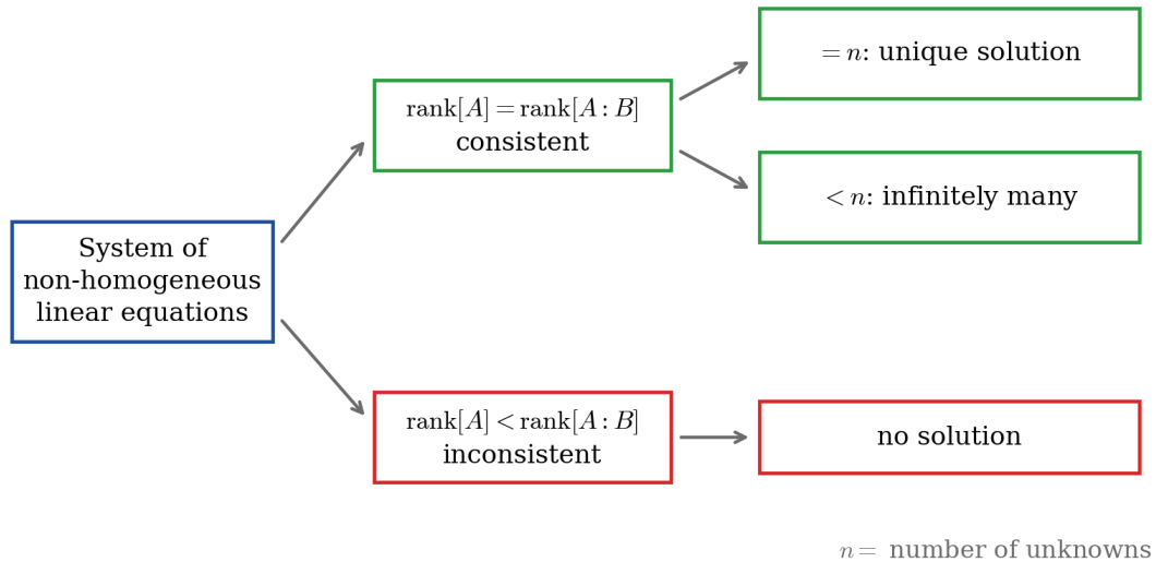
Figure 4.8.2: The rank test decides consistency first, then counts solutions.
