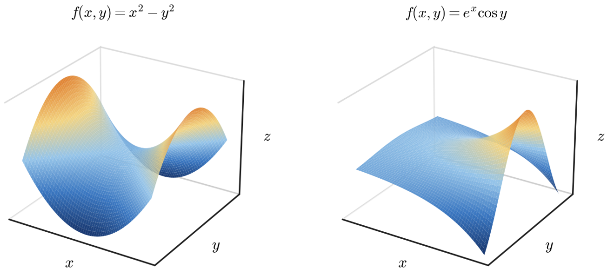
Figure 3.4.1: Two harmonic functions. Neither surface has a summit or a basin; each rises in one direction exactly as fast as it falls in the other.
