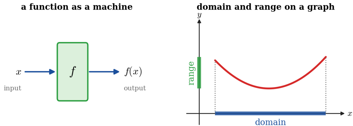
Figure 1.4.2: Left: f as a machine turning an input into an output. Right: the domain read off the horizontal axis and the range off the vertical axis.
