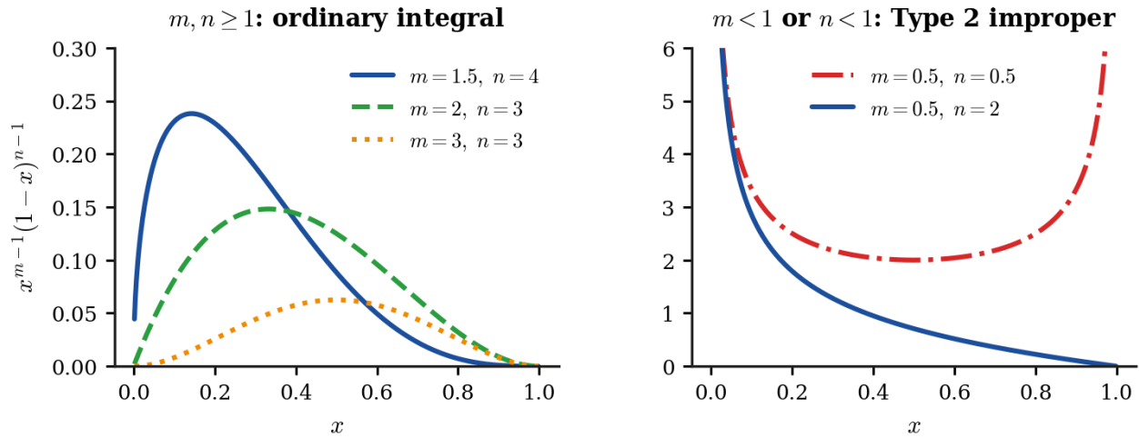
Figure 2.6.2: The beta integrand on [0, 1] . Exponents below 1 send the curve to infinity at the corresponding endpoint.
