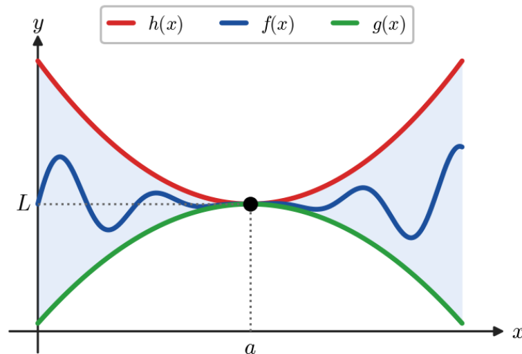
Figure 1.9.3: f is trapped between g and h , and both of those are forced to L at a ; so f has nowhere else to go.
