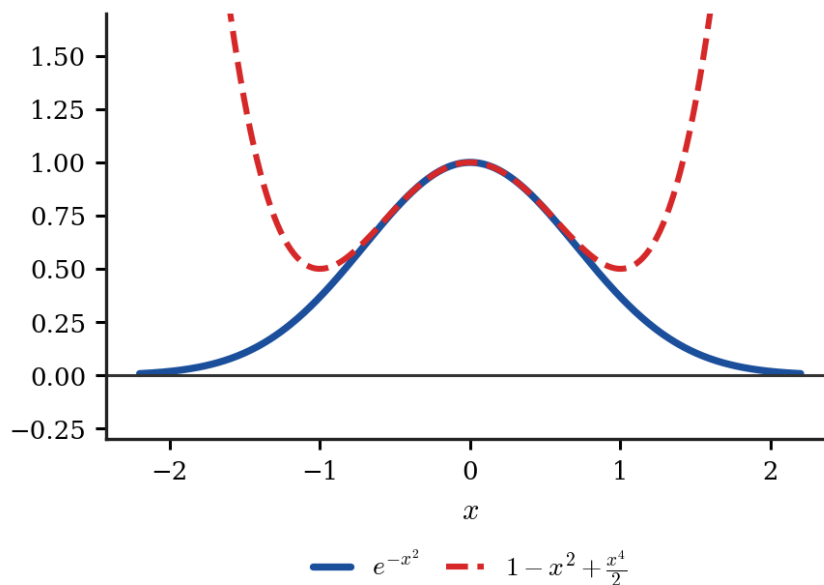
Figure 2.8.4: e^{-x^2} and its fourth degree Maclaurin polynomial. Term by term integration of the series is accurate over the range where the two curves agree.
