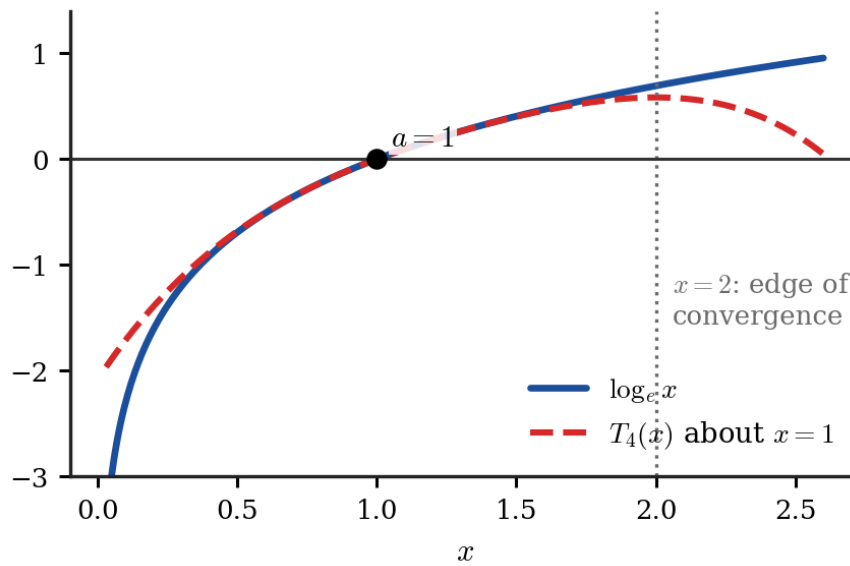
Figure 2.8.1: T_4 tracks \log_e x closely near the centre a = 1 and pulls away as x approaches the ends of (0, 2] , outside which the series does not converge.
