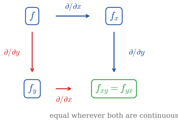
Figure 3.3.1: Either route from f to the mixed second derivative gives the same function, provided both mixed partials are continuous.
