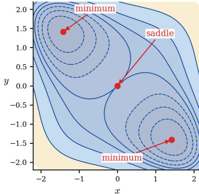
Figure 3.8.2: Level curves of f(x, y) = x^4 + y^4 - 2x^2 + 4xy - 2y^2 with its three critical points. The two off-origin points sit at the centres of closed curves; the origin lies where two level curves cross.
