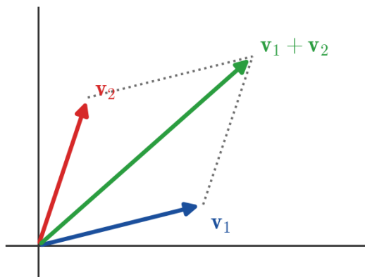
Figure 4.9.1: Two vectors in the plane. Independent vectors point in genuinely different directions and together reach every point of the plane; dependent ones lie along a single line, so one is a multiple of the other.
