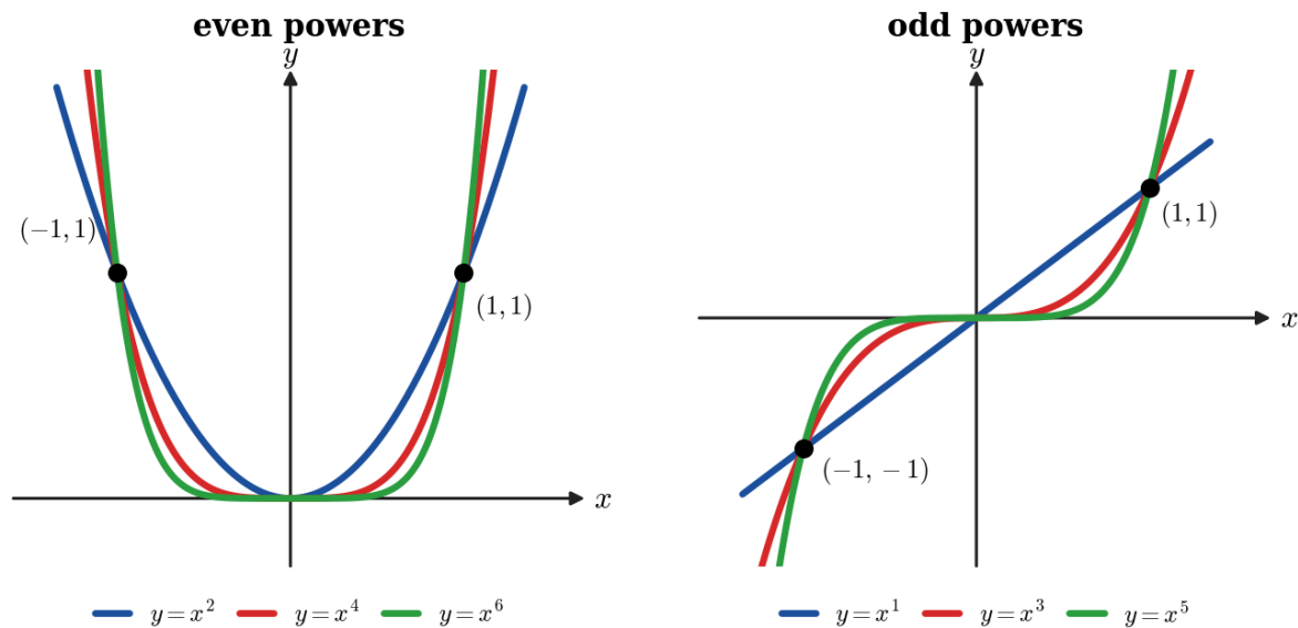
Figure 1.5.1: All these curves pass through (1, 1) , and through (-1, 1) or (-1, -1) according to whether the power is even or odd. The larger the exponent, the flatter the curve near the origin and the steeper beyond |x| = 1 .
