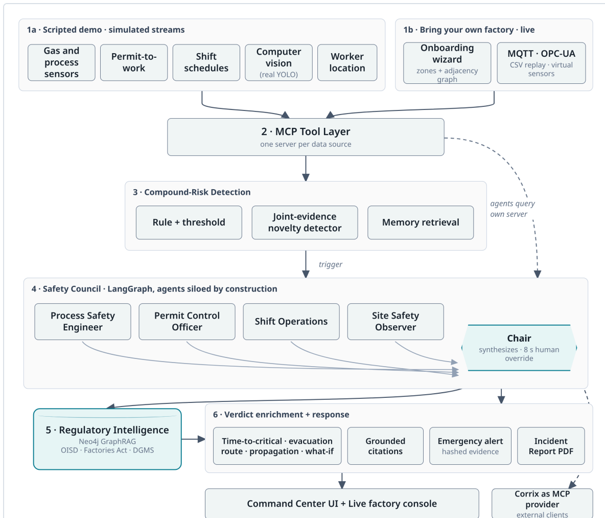
Figure 1. The Corrix system: one reasoning engine, two front doors, six layers.
