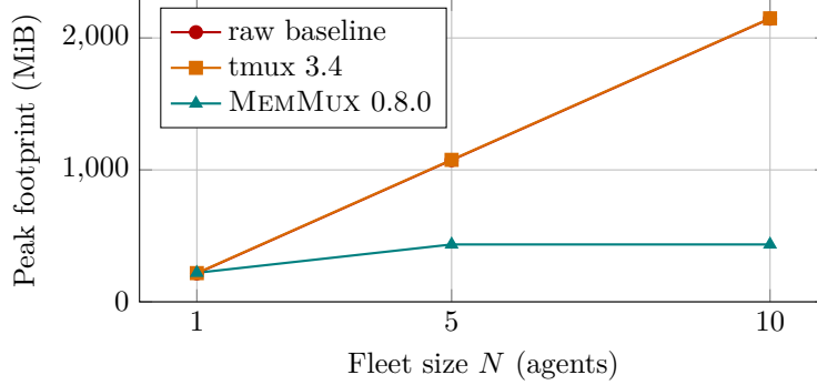
Figure 1: Peak fleet footprint under a 3000 MiB budget ( overcommit ). Ungoverned tools scale linearly with the fleet; MEMMUX stays flat by deferring admissions ( 4.9\times lower at N=10 ).
