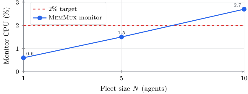
Figure 4: Cost of the always-on 1 Hz attribution scan (H5), the paper’s honest weak spot. Overhead is linear in the process count and crosses the 2% target between five and ten agents; incremental sampling is the planned fix. The baselines run no such monitor.
