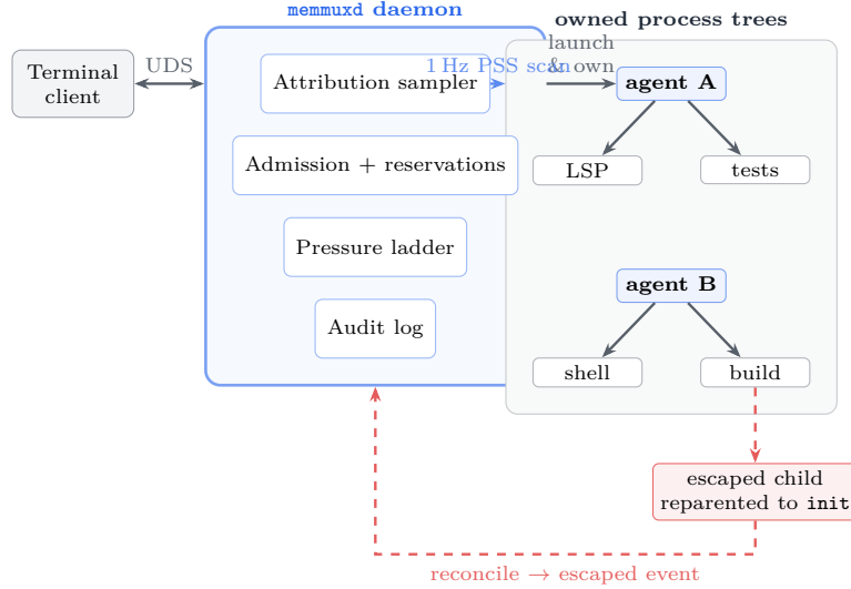
Figure 1: MEMMUX architecture. A terminal client drives the memmuxd daemon over a Unix domain socket. The daemon launches and owns each agent’s process tree; a 1 Hz sampler sums proportional memory (PSS) across every owned subtree (H1), reconciliation flags any child that double-forks out to init (H3), and admission, the pressure ladder, and an audit log turn the budget into checkable, logged decisions (H2/H4/H5).
