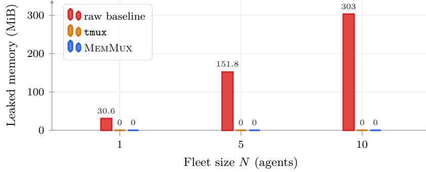
Figure 3: Memory stranded ten seconds after normal teardown ( hold ). The raw baseline kills only the roots, so it leaks a grandchild per agent—half of every fleet, growing to 303 MiB at N=10 (50% reclaimed). tmux and MEMMUX reap their full subtree at every size (0 leaked, 100% reclaimed).
