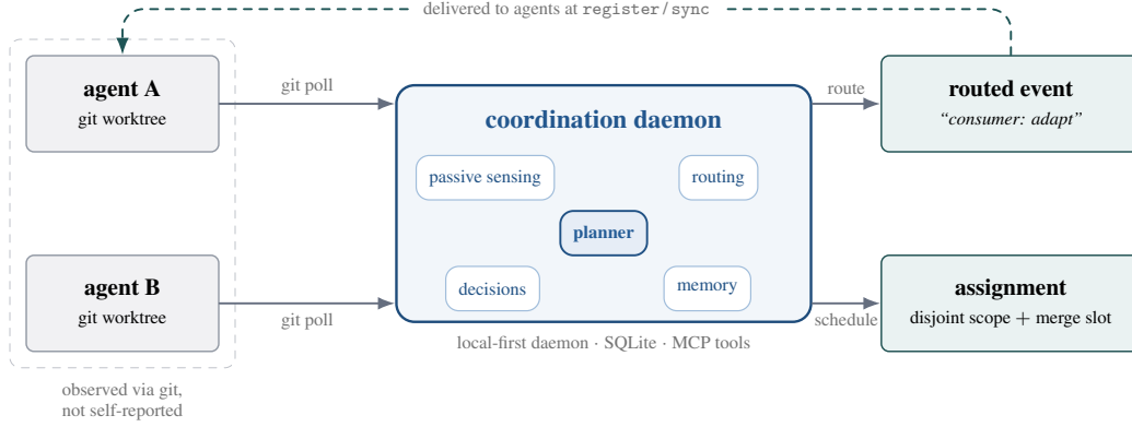
Figure 1: our coordination plane observes each agent’s worktree by polling git ( passive sensing ), then routes only the relevant events and—with the planner—hands each agent a disjoint scope and a merge slot before the edits happen, rather than warning after a collision is sensed.
