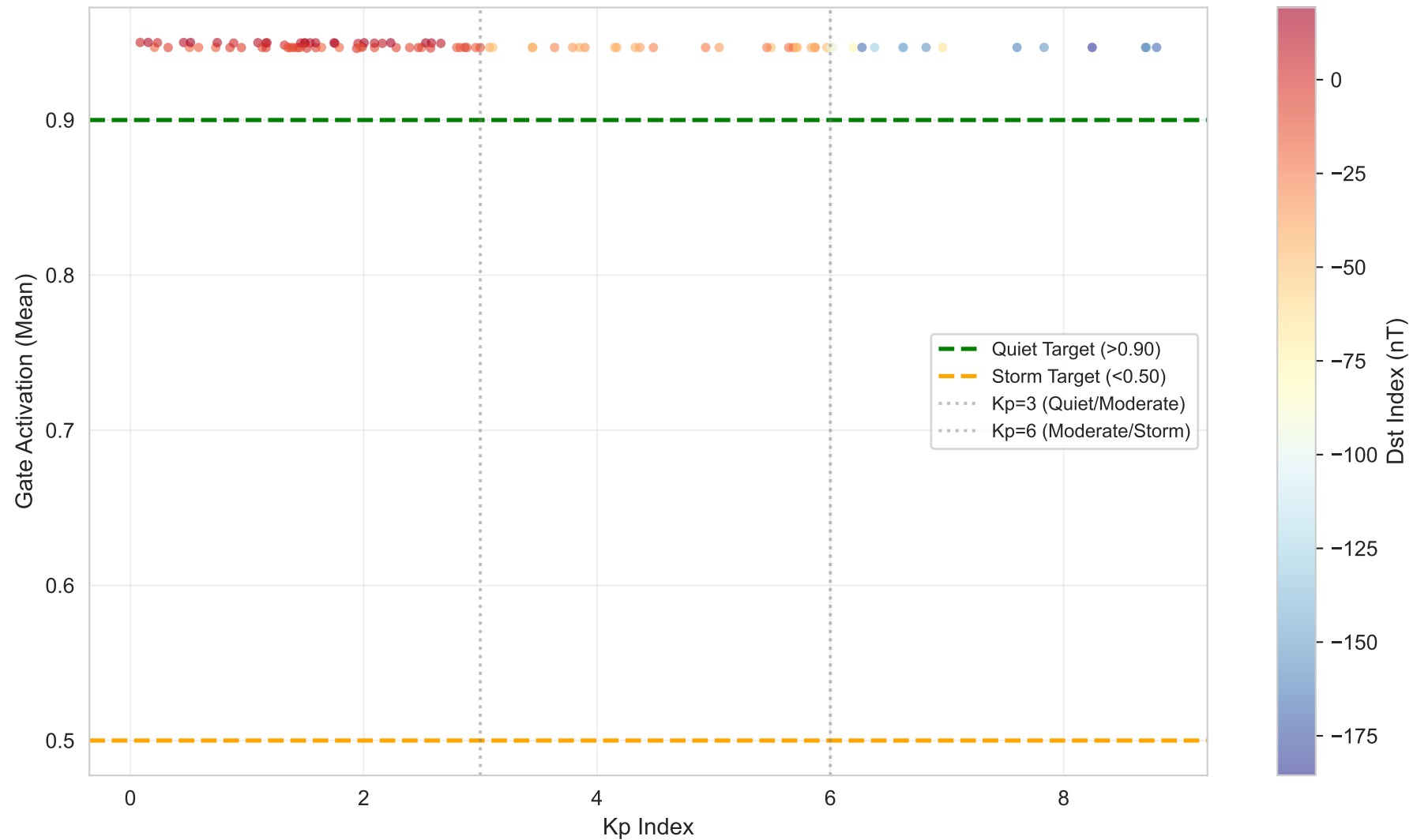
S01: Cosmic Gate Activation vs Kp Index
