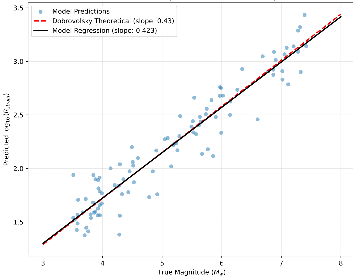
S04: Dobrovolsky Strain Radius Consistency
