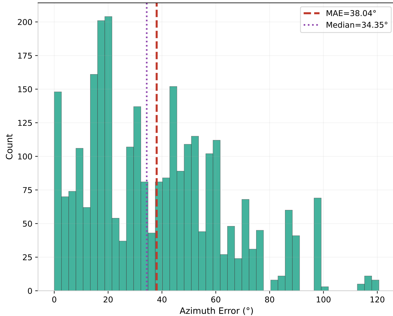
Azimuth Error Distribution
