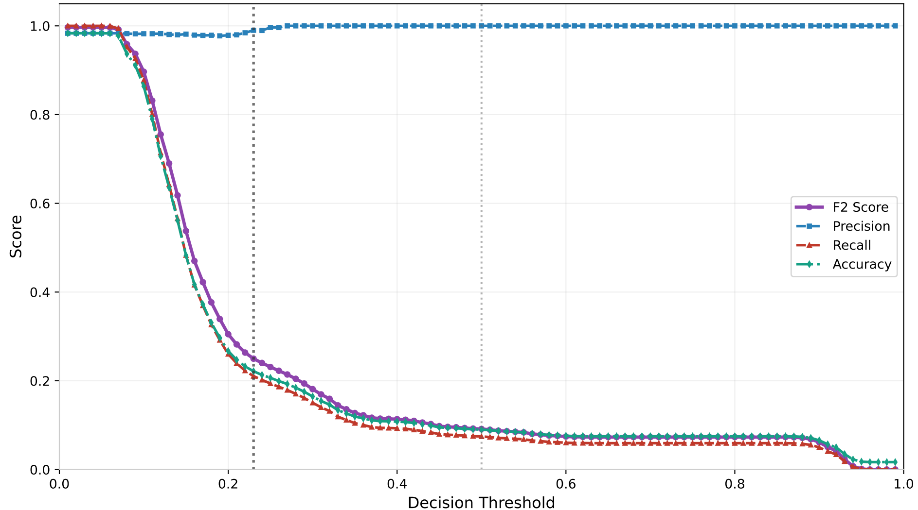
V8 SupCon — Threshold Performance Analysis
