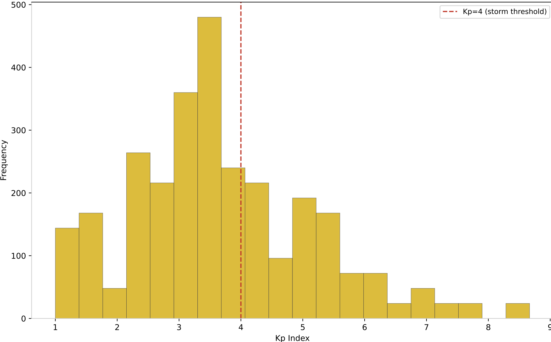
Kp-Index Distribution
