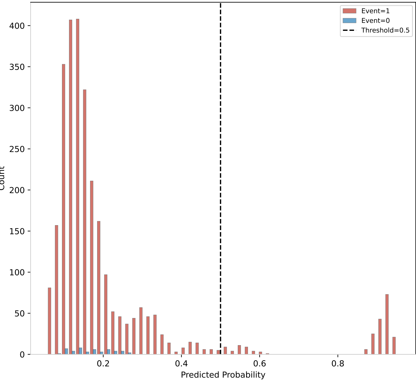
Prediction Probability Distribution
