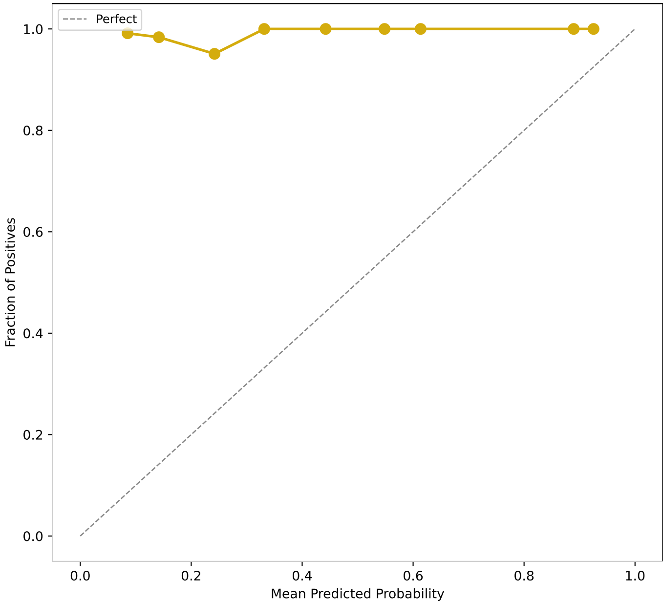
Calibration Curve
