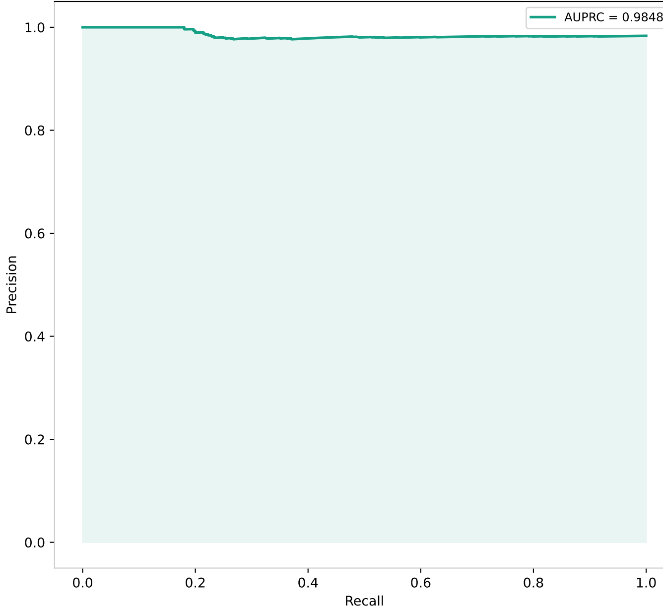
Precision-Recall Curve
