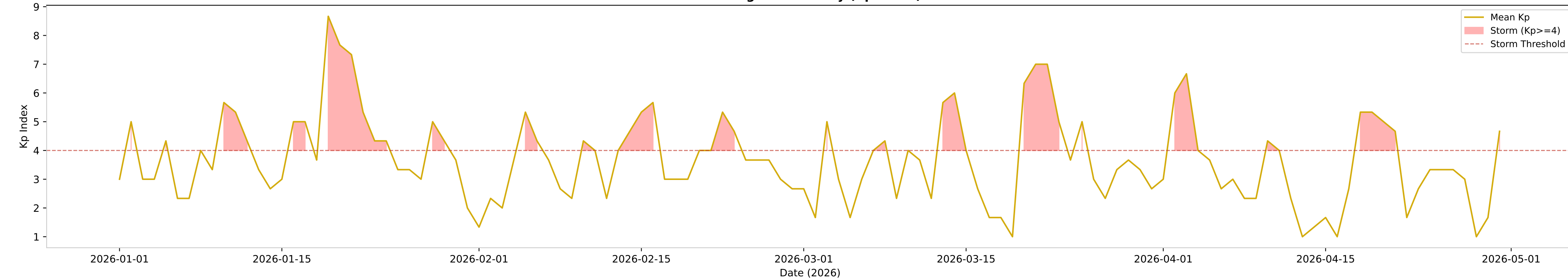
Geomagnetic Activity (Kp-index)
