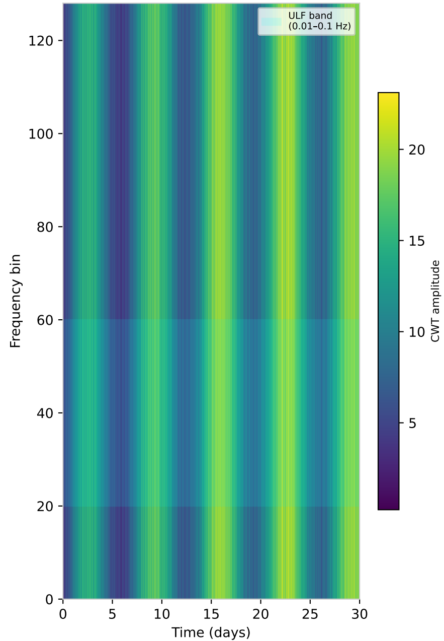
A. Original CWT Scalogram (tectonic anomaly)
