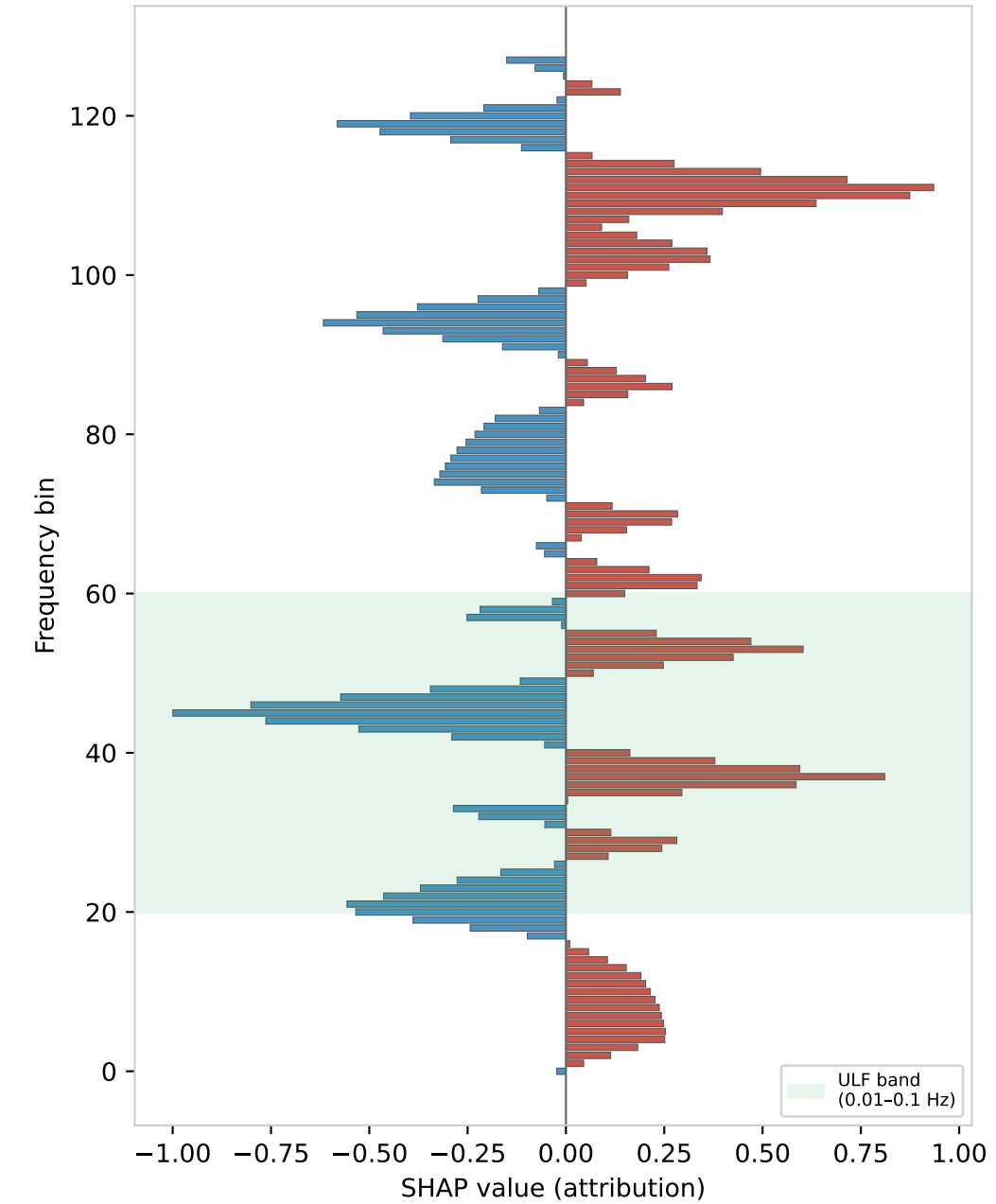
C. SHAP Frequency Feature Importance
