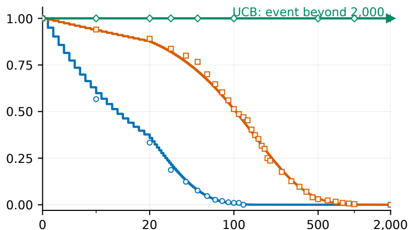
(c) First revisit; gap D = 1
