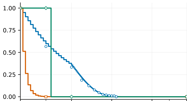
(a) First revisit; gap D = 0.01
