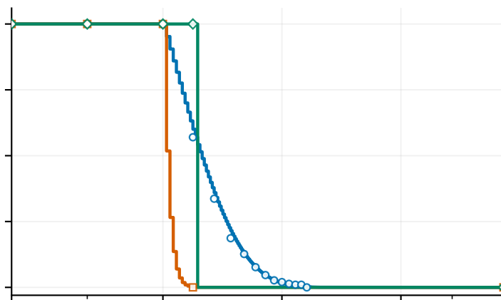
(b) Confirmed Q recovery; gap D = 0.01
