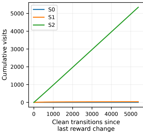
(c) State visits
