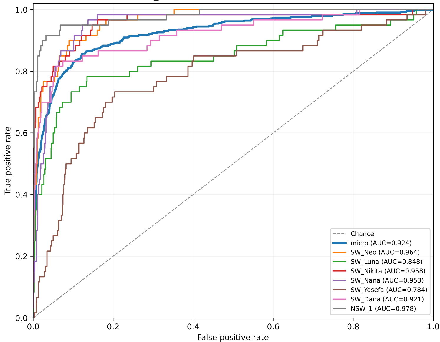
aves_bio — detection ROC on held-out test
