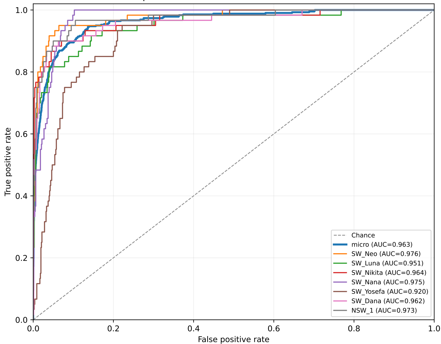
dolph2vec — detection ROC on held-out test
