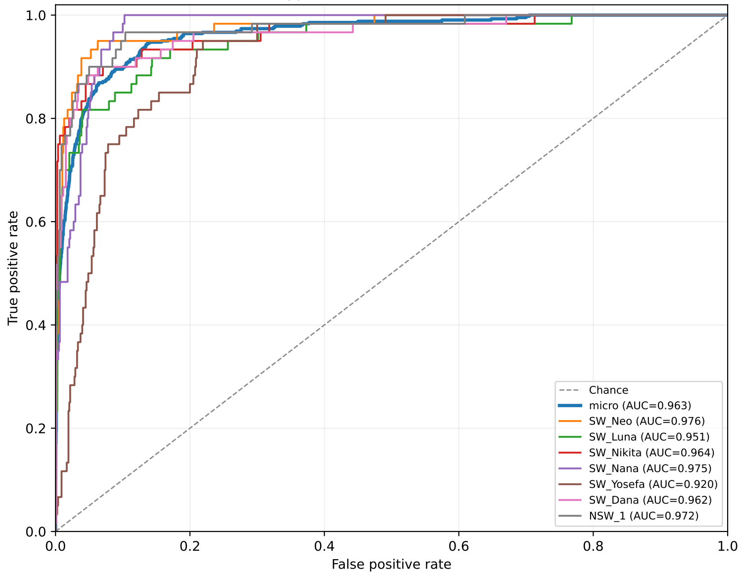
Whistle-type detection ROC on held-out test
