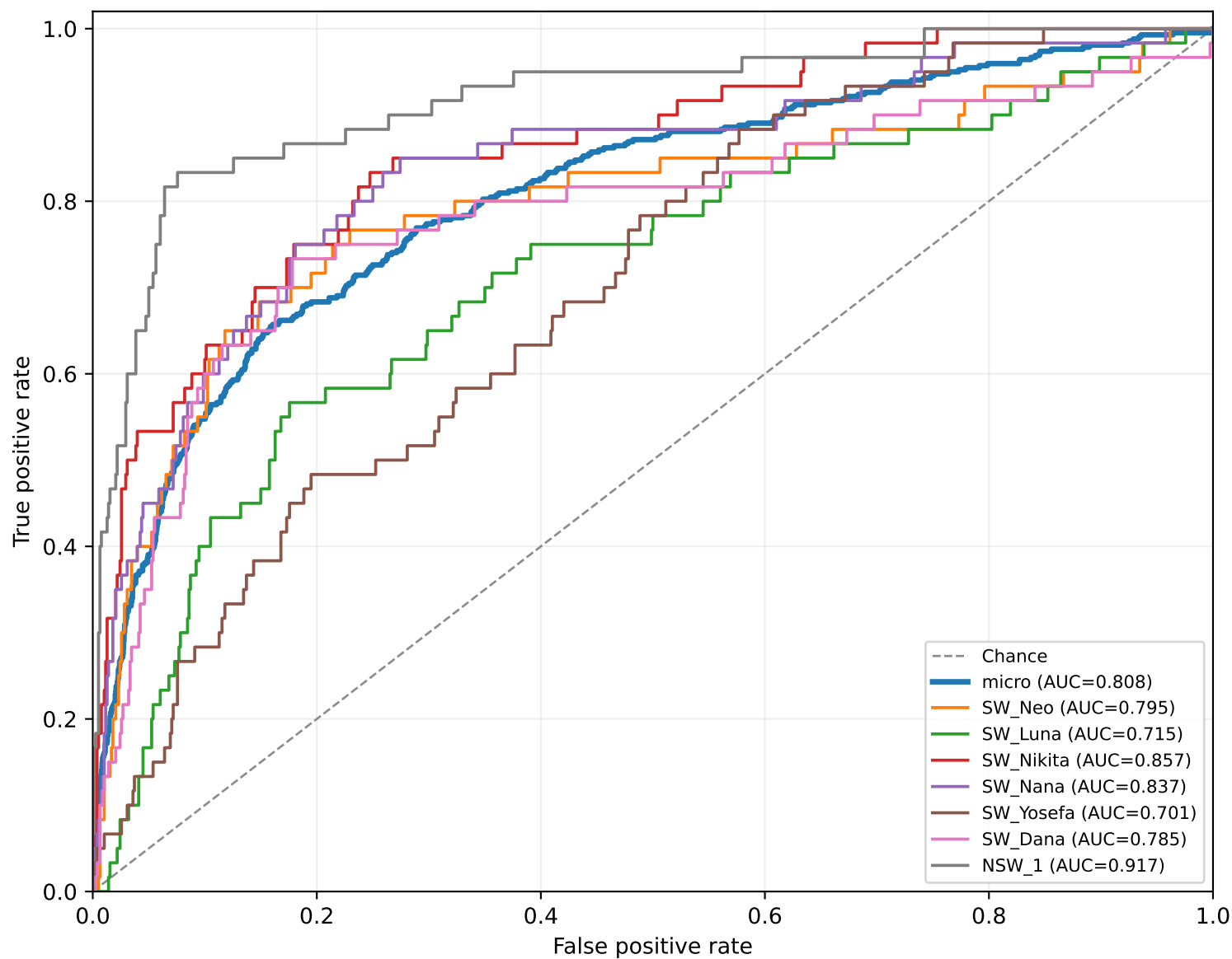
mfcc — detection ROC on held-out test
