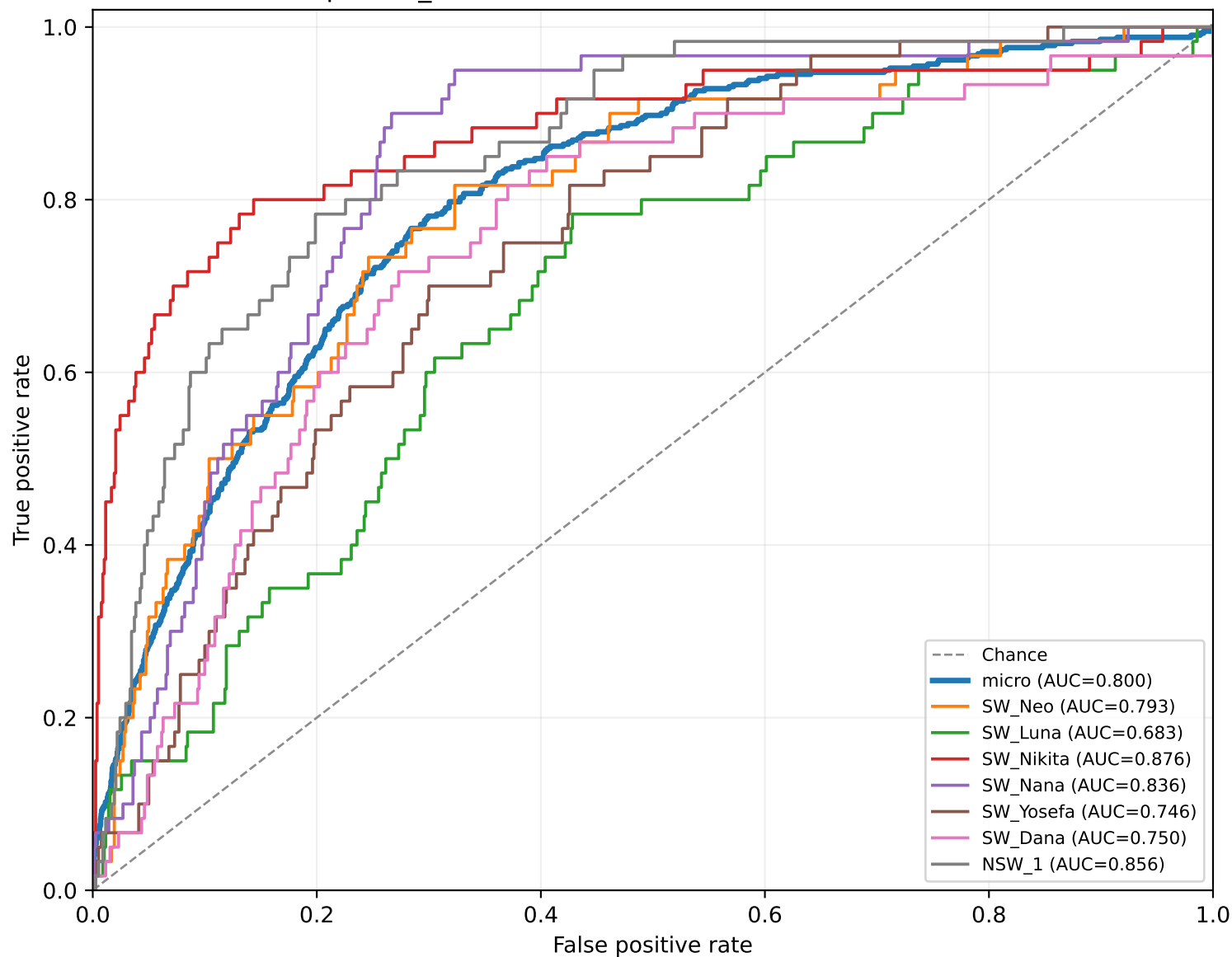
spectral_features — detection ROC on held-out test
