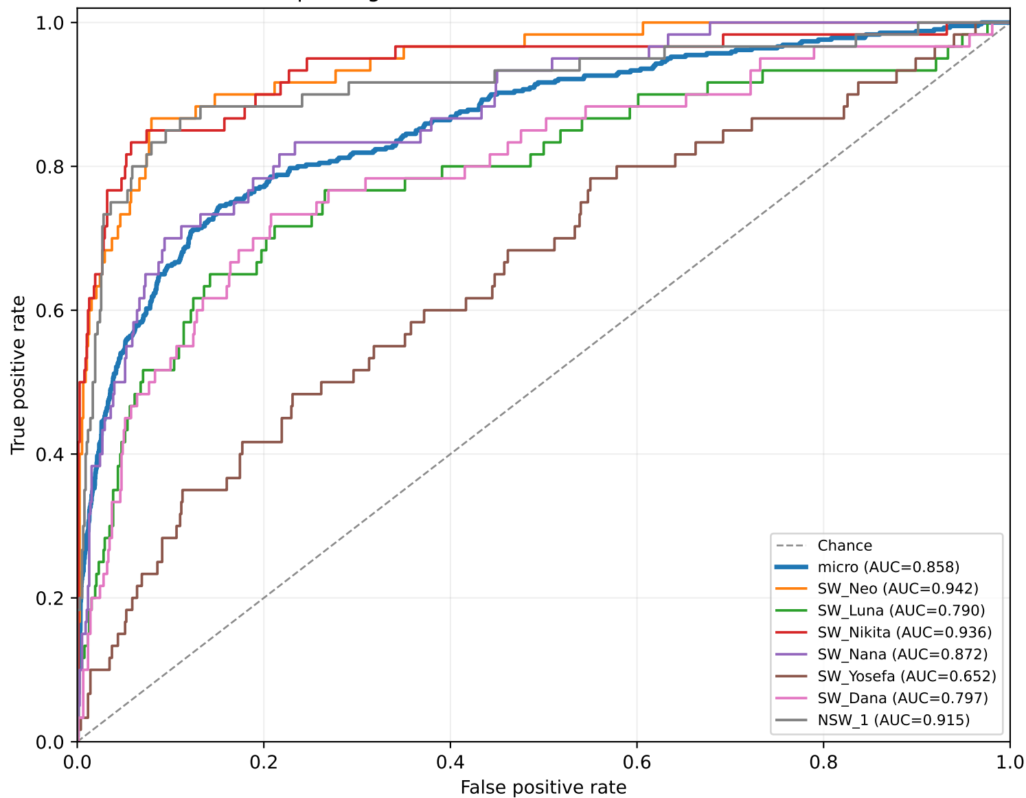
spectrogram — detection ROC on held-out test
