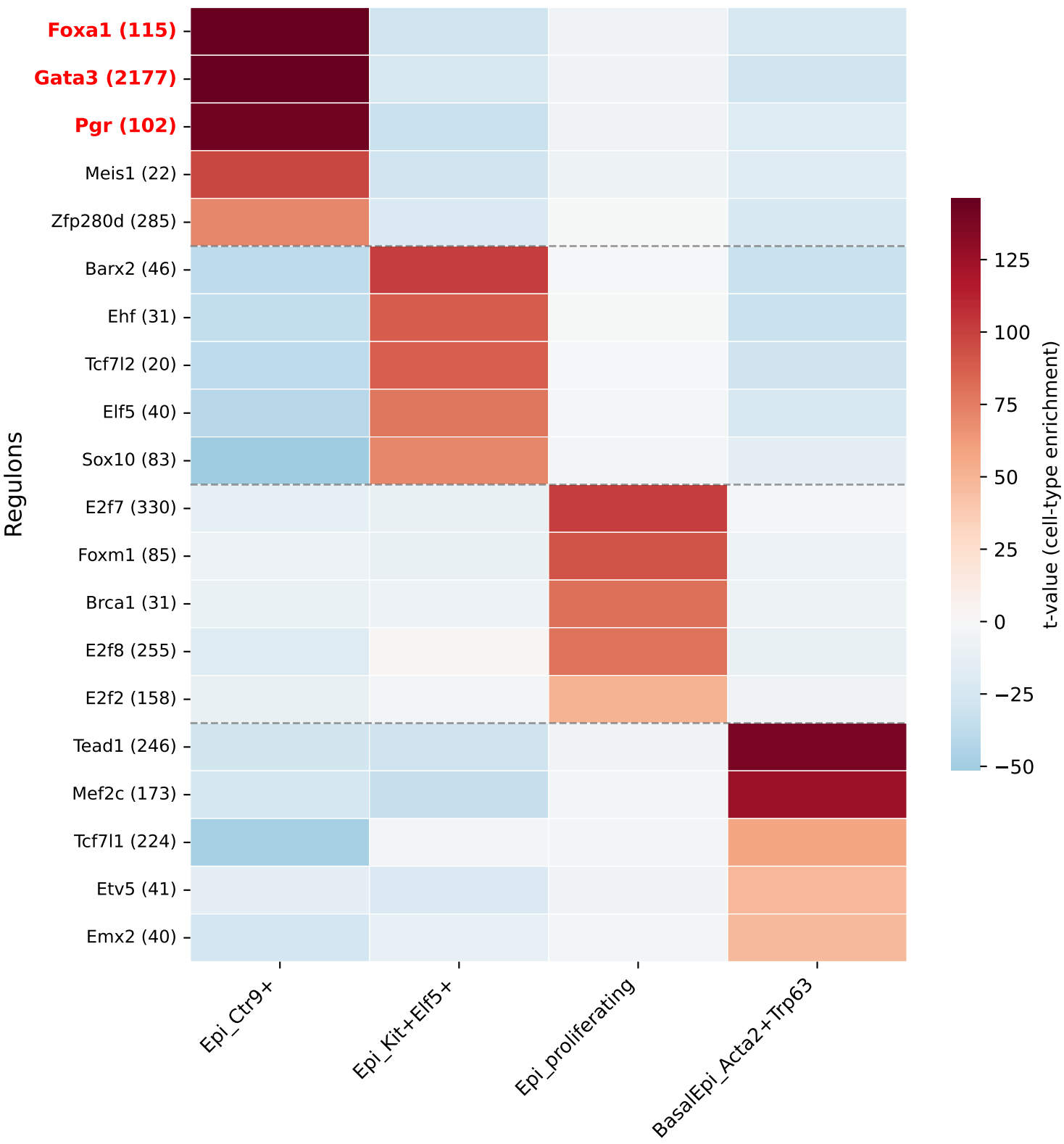
Regulon Activity in Epithelial Populations (top 5 per population, one-vs-rest t-values controlling for condition)
