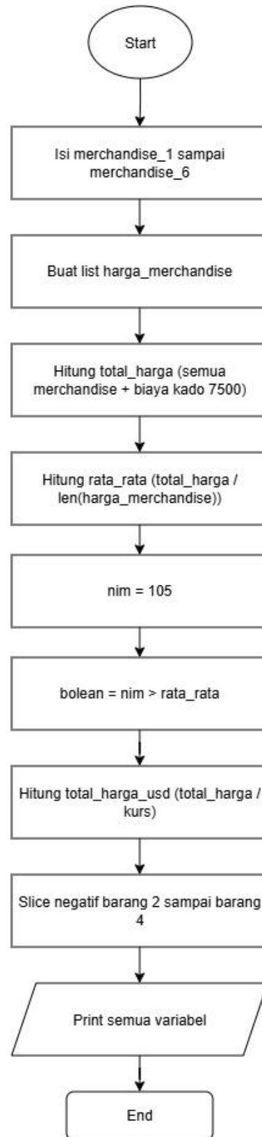
Gambar 1.1 Flowchart
