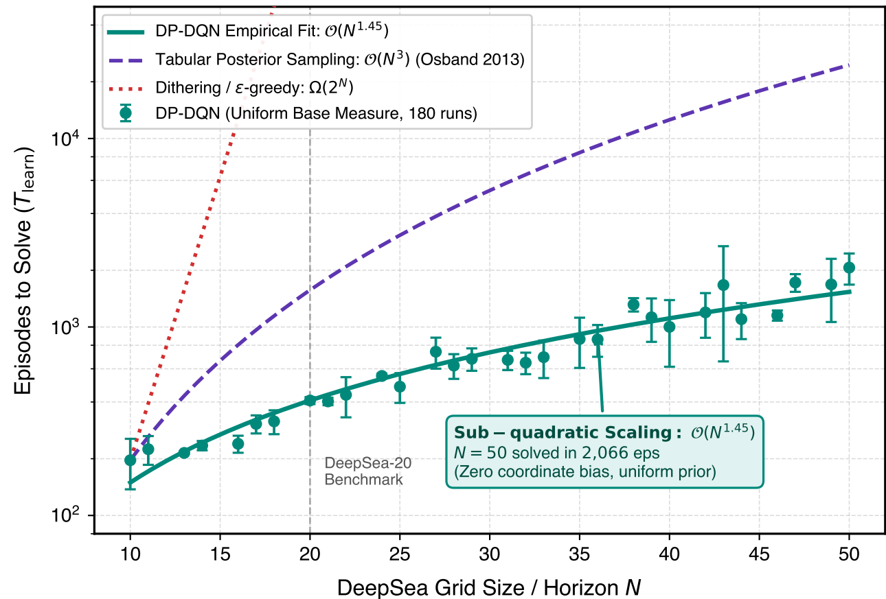
(b) Scalability Across Horizon N \in [10, 50]
