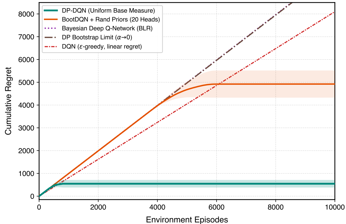
(a) DeepSea-20 Cumulative Regret (10 Seeds)
