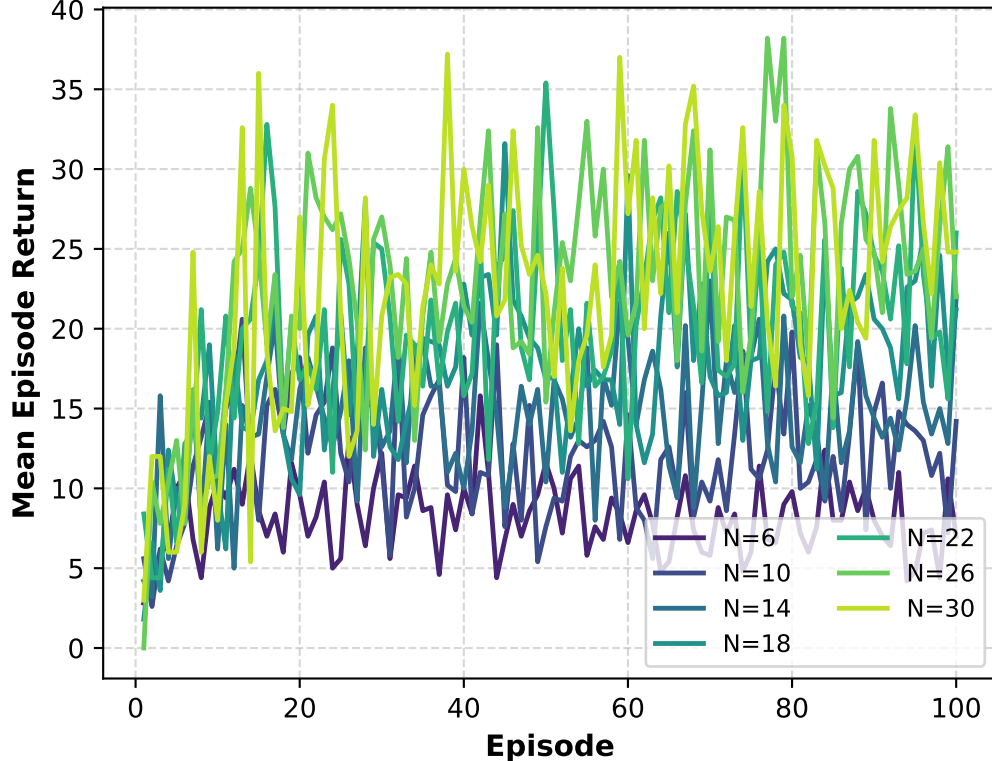
(b) Learning Curves Across River Lengths
