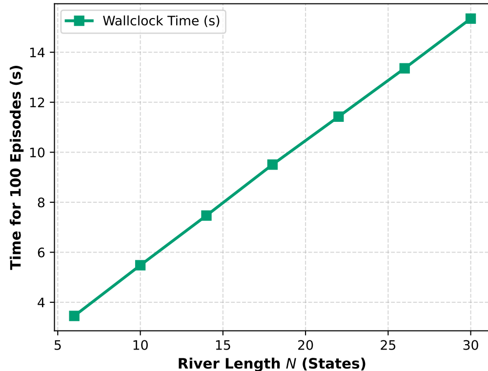
(c) Wallclock Computation Scaling
