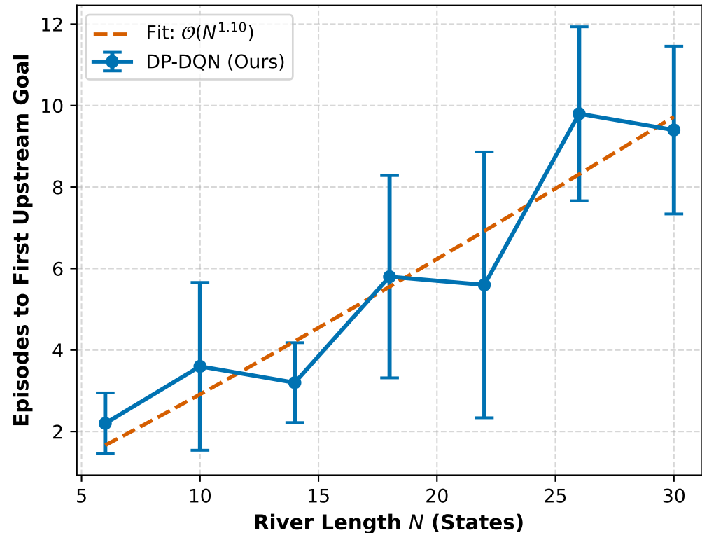
(a) Sample Complexity Scaling on RiverSwim
