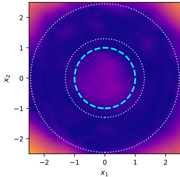
B. Deep Ensembles (Gaussian NLL)
