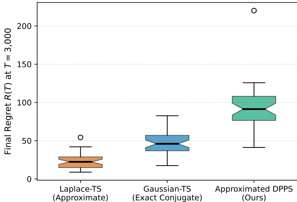
(b) Final Regret Dispersion Across 40 Seeds
