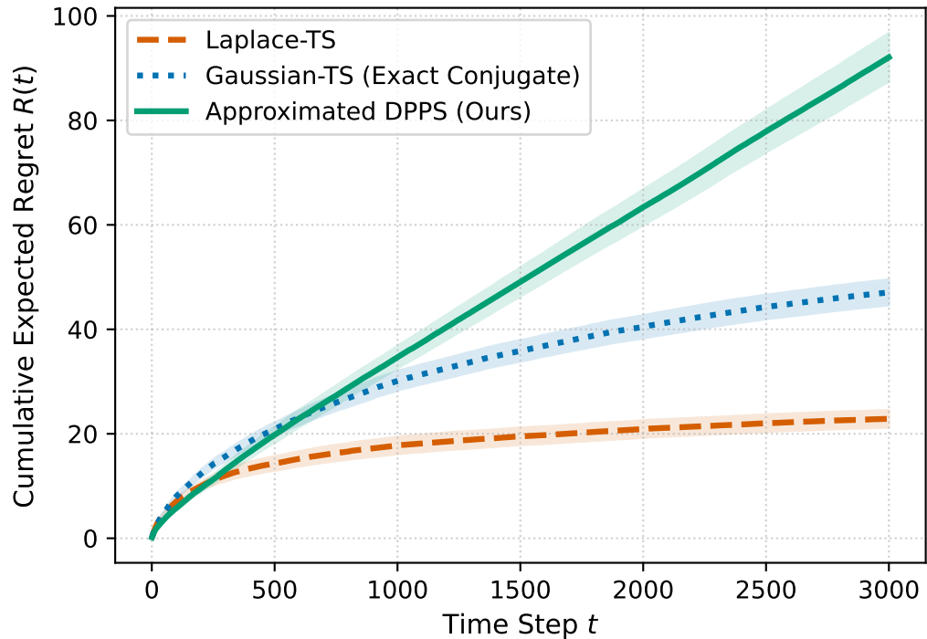
(a) Cumulative Regret on Logistic Bernoulli Bandit
