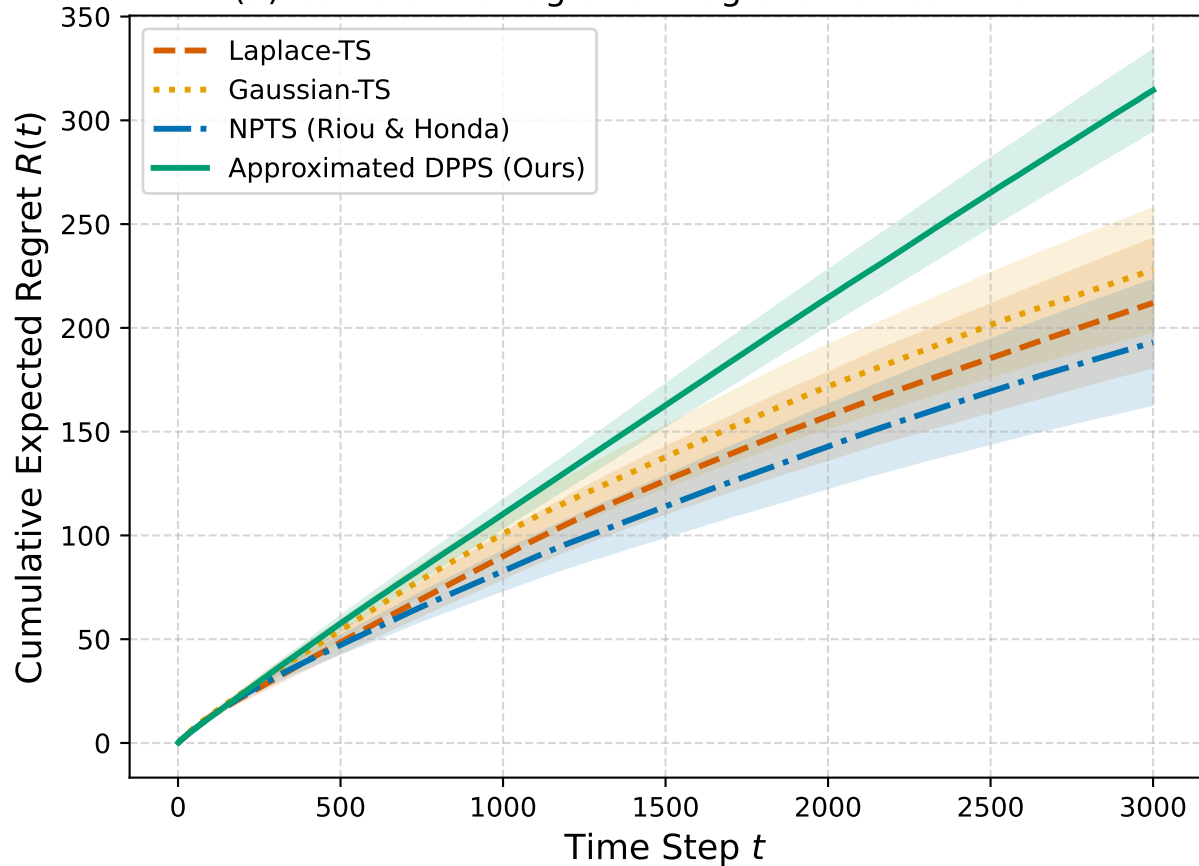
(a) Cumulative Regret on Logistic Bernoulli Bandit
