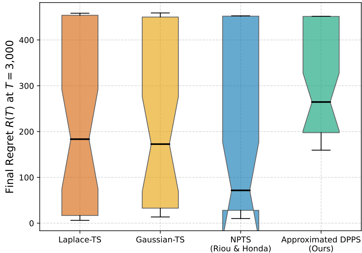
(b) Final Regret Dispersion Across 40 Independent Runs
