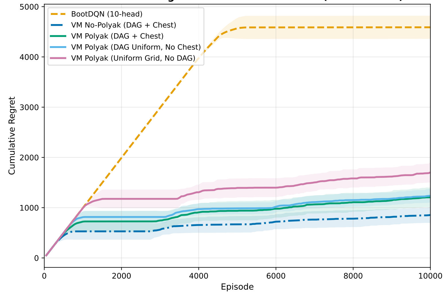
A. Cumulative Regret Across Base Measures (Mean \pm 1 SD)
