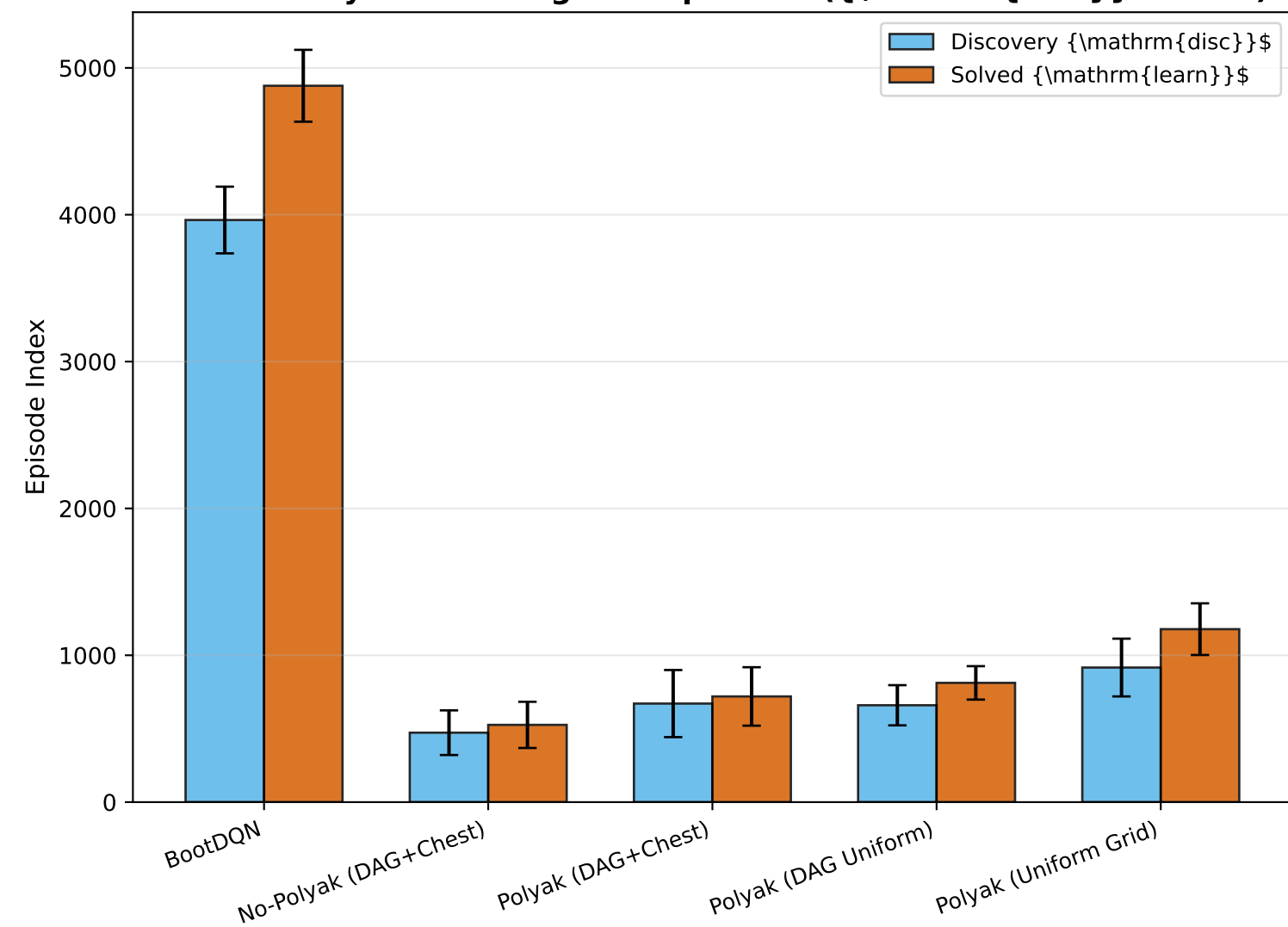
C. Discovery vs. Convergence Episodes ( \{\mathrm{disc}\} vs. \{\mathrm{learn}\} )
