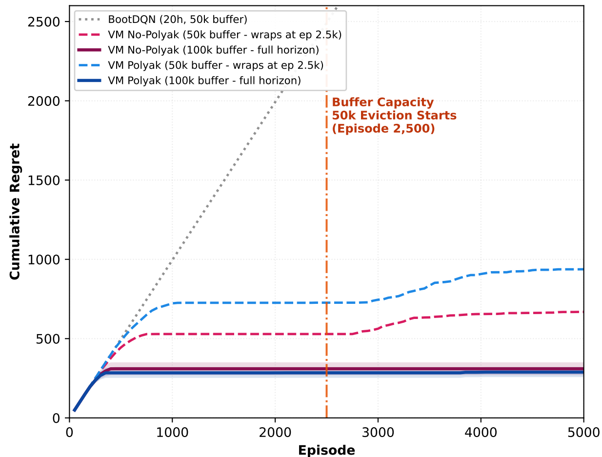
Cumulative Regret on Deep Sea 20×20 (50k FIFO Eviction vs. 100k Full Horizon)
