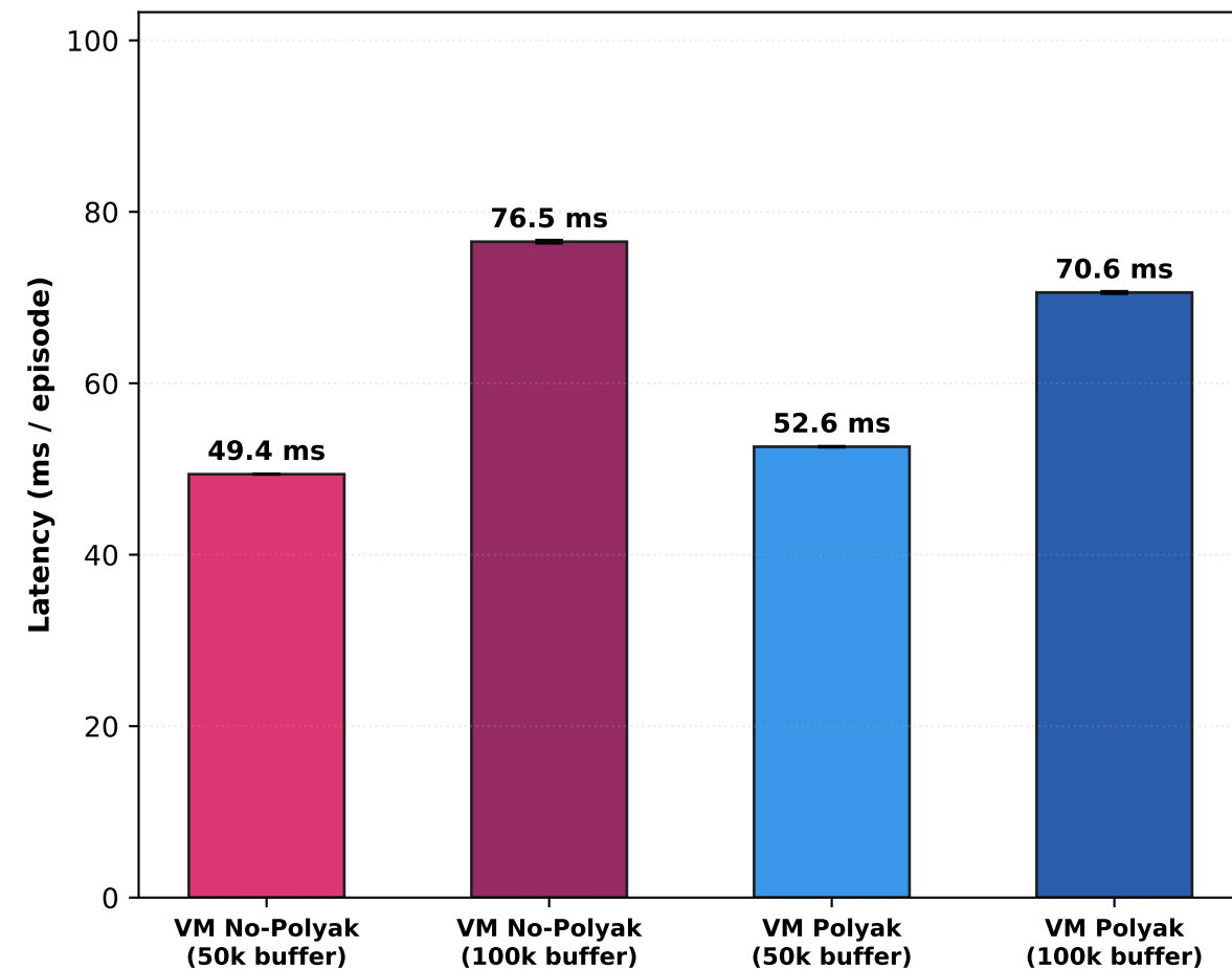
Computational Cost Verification (Zero Overhead: 50k vs. 100k Buffer)
