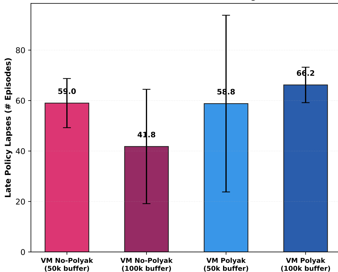
Post-Discovery Policy Lapses (Elimination of FIFO Detuning)
