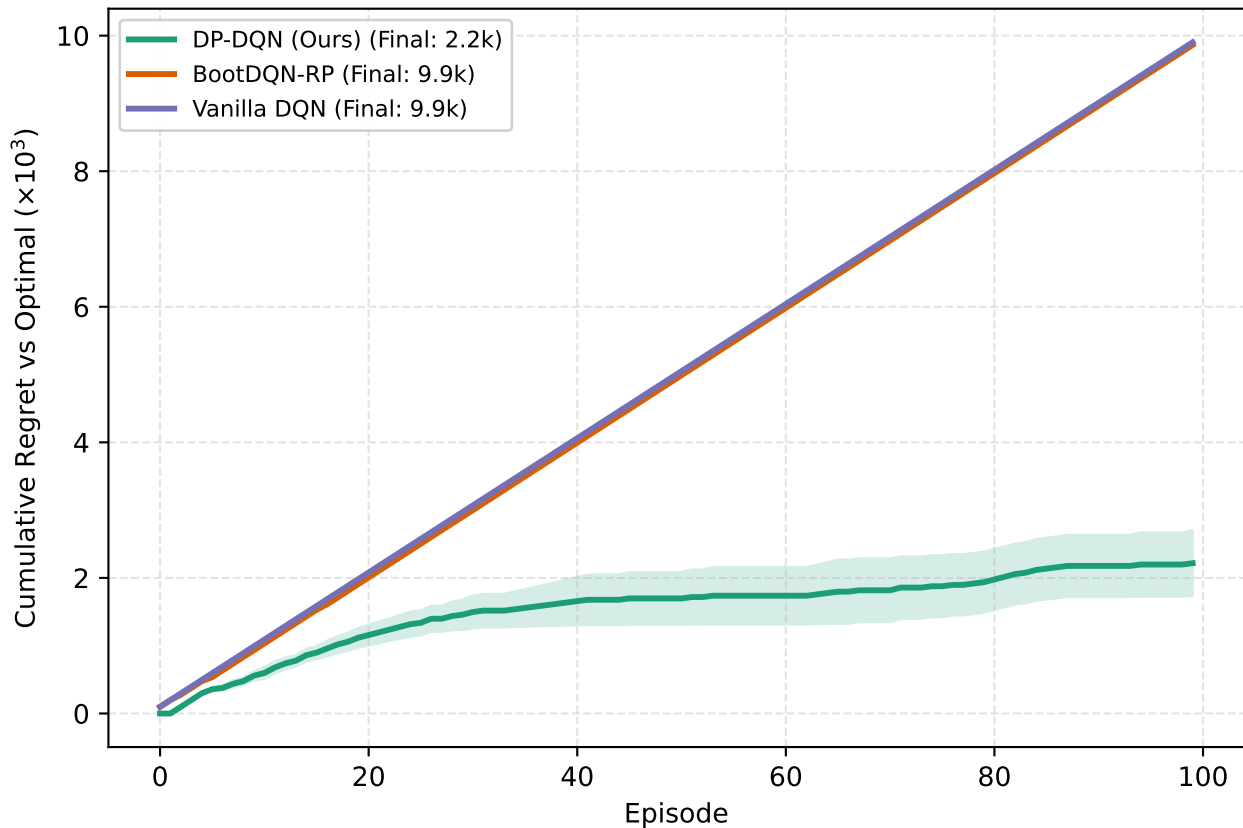
(a) Deceptive N-Chain ( N = 20 ): Cumulative Regret
