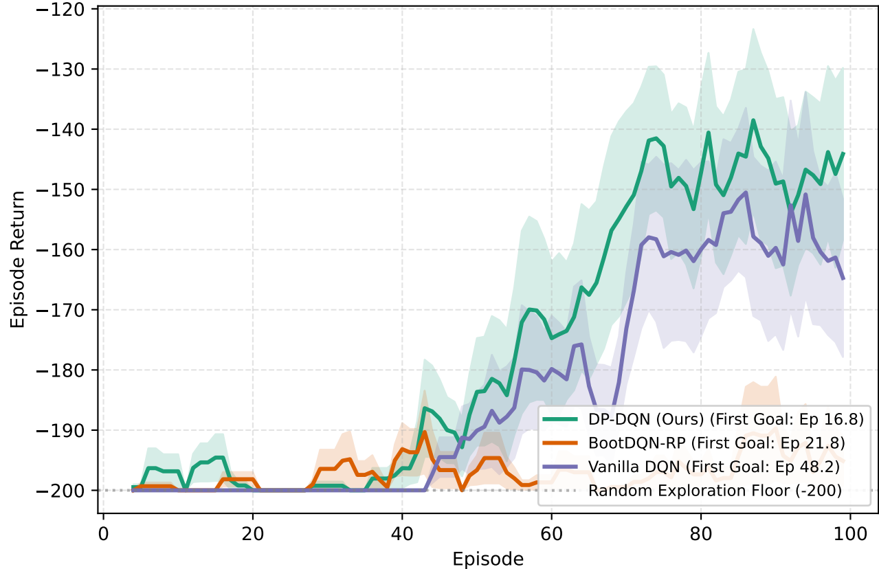
(b) MountainCar-v0: Episode Return (5-step avg)
