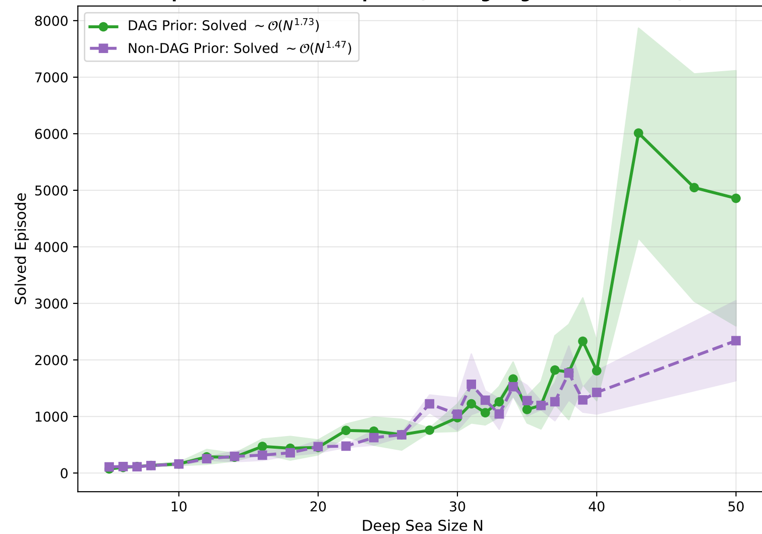
Episodes to Solve Deep Sea (Moving Avg Return \geq 0.85 )
