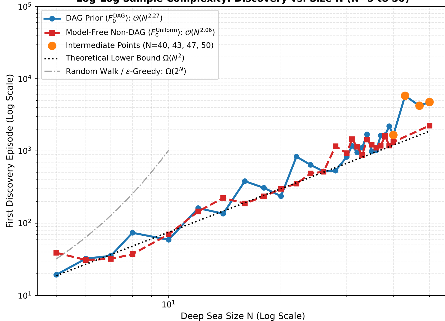
Log-Log Sample Complexity: Discovery vs. Size N (N=5 to 50)
