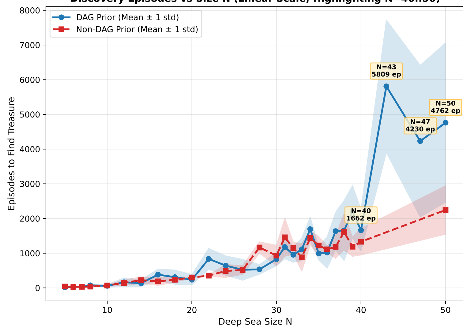
Empirical Scaling Proof across Intermediate Sizes [40, 50]
