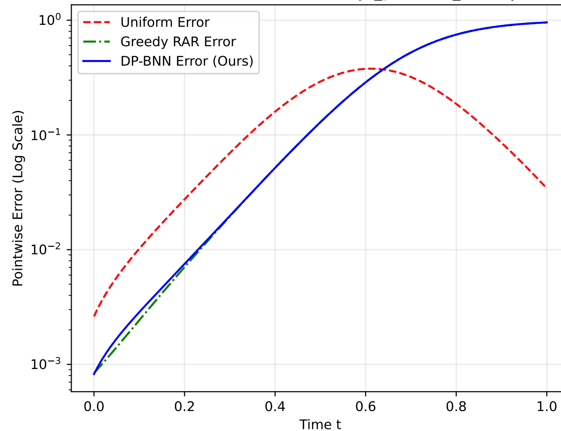
(b) Absolute Error Profile |u_{\text{pred}} - u_{\text{exact}}|
