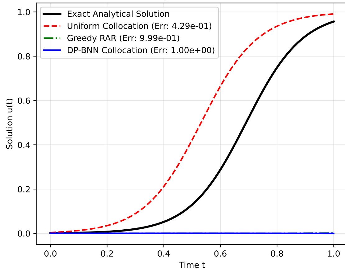
(a) Solution Comparison on Stiff Wavefront
