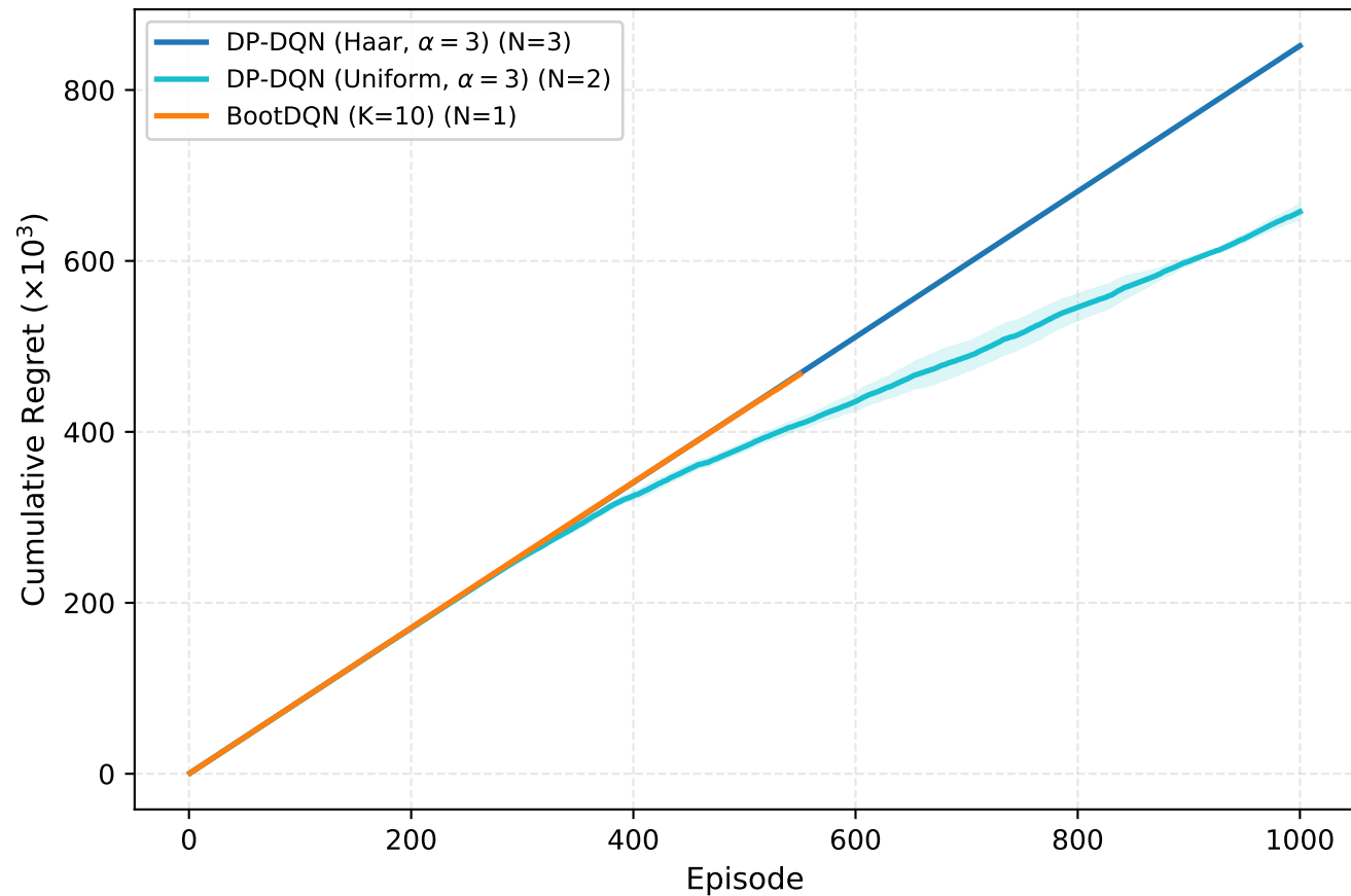
Cumulative Regret (Live: Ep 1-1000)
