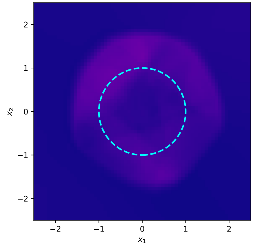
C. Variational BNN (BBB) [Catastrophic Cavity Collapse]
