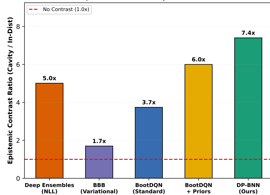
F. Epistemic Uncertainty Contrast Ratio
