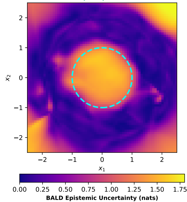
E. DP-BNN (Ours: Measure Prior) [Clean Isotropic Epistemic Bubble!]
