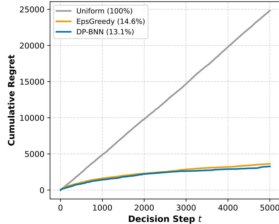
(b) Mushroom ( d = 117, K = 2 )
