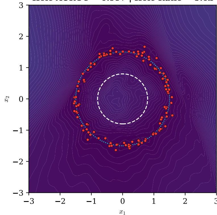
(b) Vanilla Bootstrap Hole AUROC = 0.997 | Hole Ratio = 5.0x
