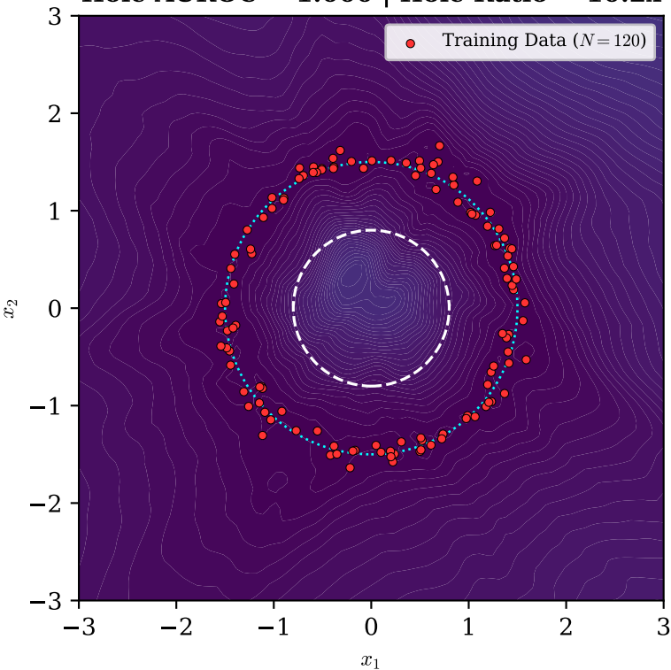
(a) Deep Ensembles Hole AUROC = 1.000 | Hole Ratio = 10.2x
