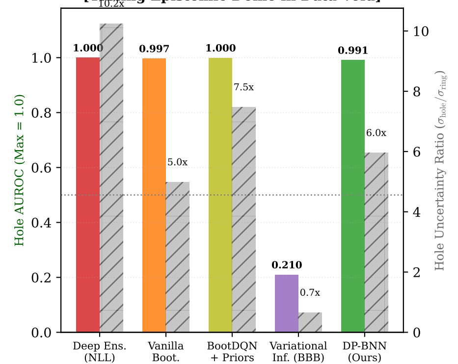
(f) Interior Hole Detection Benchmark [Testing Epistemic Dome in Data Void]
