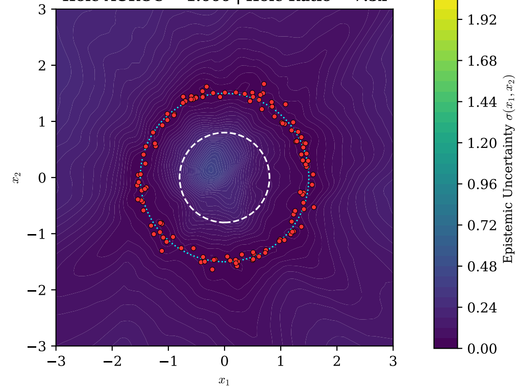
(c) BootDQN + Priors Hole AUROC = 1.000 | Hole Ratio = 7.5x
