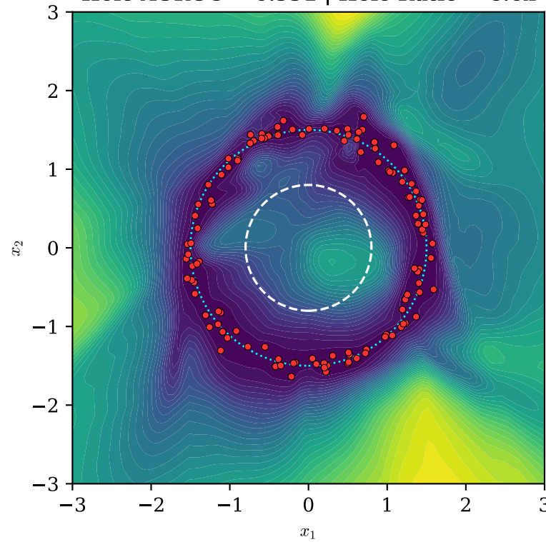
(e) DP-BNN (Ours) Hole AUROC = 0.991 | Hole Ratio = 6.0x
