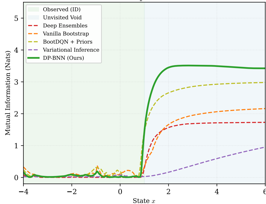
(a) Epistemic Mutual Information (BALD)
