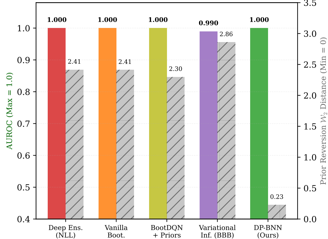
(c) Bayesian Uncertainty Benchmark
