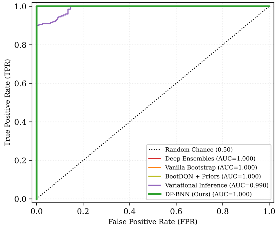
(b) Unvisited State Discrimination (ROC)
