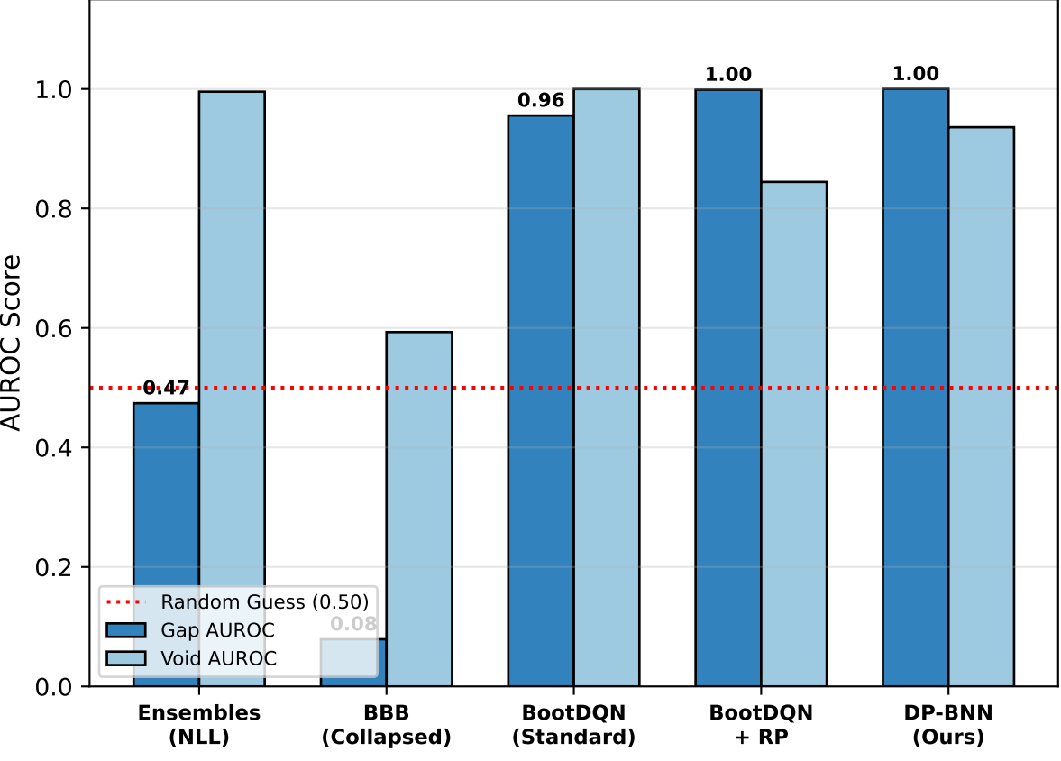
OOD AUROC under Heteroscedastic Noise
