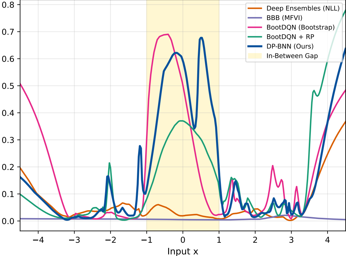
BALD Information (nats) across Domain
