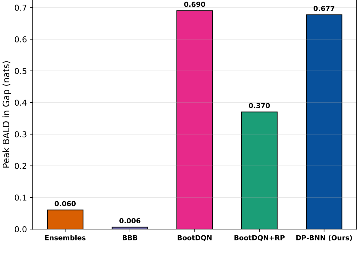
Epistemic Exploration in Gap (Higher = Better)
