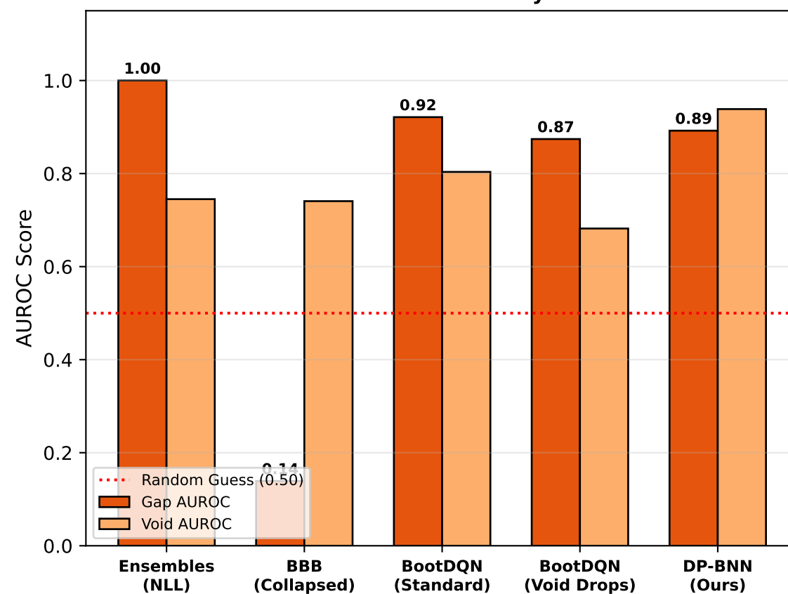
OOD AUROC under Cauchy Outliers
