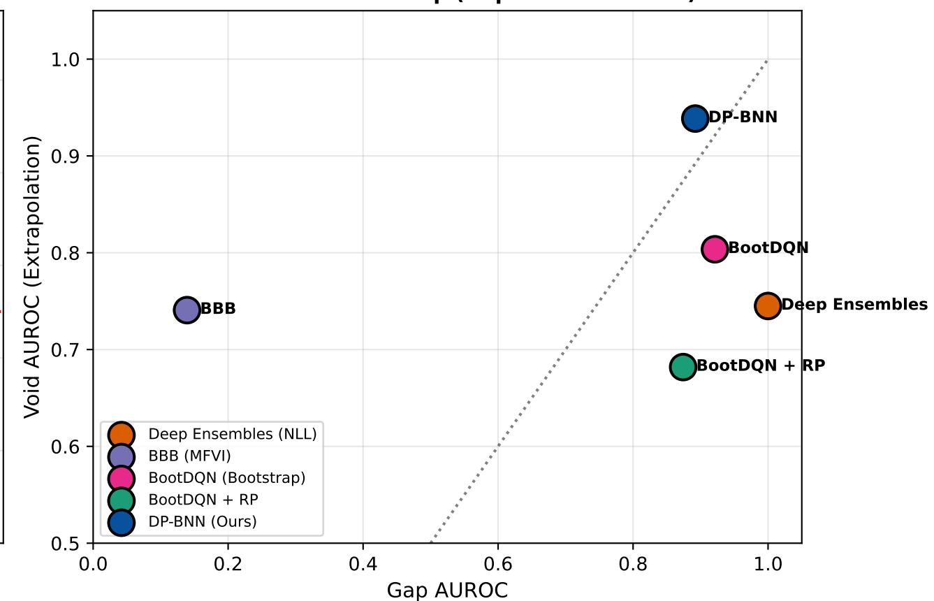
Dual Robustness Map (Gap vs Void AUROC)
