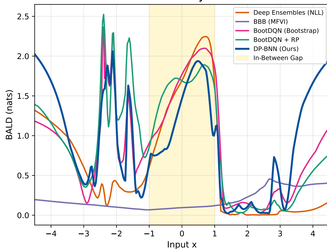
BALD Information under Cauchy Outlier Contamination
