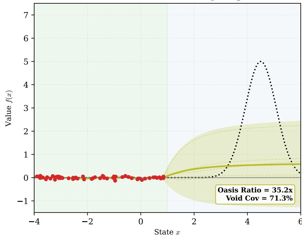
(b) Standard BootDQN + Priors (Unconstrained Gaussian — Dips negative)
