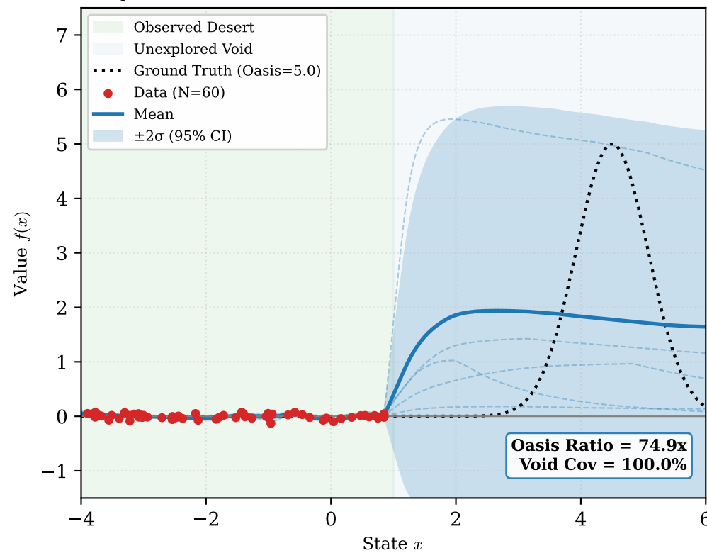
(a) DP-BNN: Positive Gaussian Prior ( y \geq 0 , UNBOUNDED ABOVE — No 5.0 assumed!)
